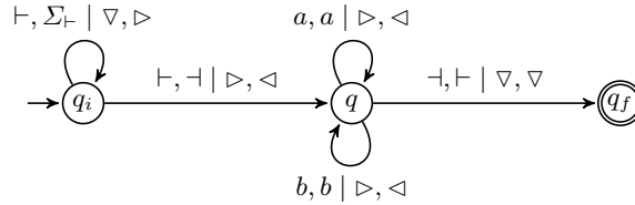
Fig. 2. Automaton recognizing \{(u, \tilde{u}) \mid u \in \Sigma^*\} when \Sigma = \{a, b\}
