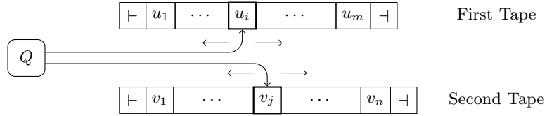
Fig. 1. Schema of a two-way two-tape finite automaton
