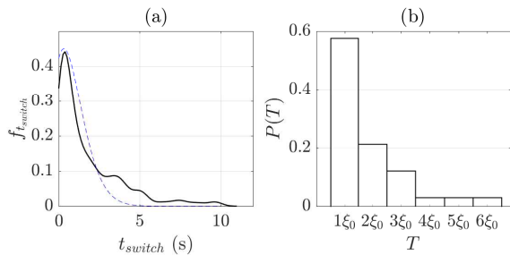
FIG. 17. (a) PDF of the switching time t_{switch} for the raw data (black solid line) together with a Poisson distribution (parameter set to 0.86, blue dashed line) and (b) probabilities of switching at times T multiple to \xi_0 = 4.3 for the LP filtered signal.
