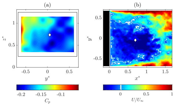
FIG. 2. Typical (a) instantaneous pressure field over the rear part of the model and (b) instantaneous 2D velocity field in the horizontal plane shown on Fig. 1. The diamond (white) is the instantaneous barycenter position of respectively (a) the rear pressure G_p and (b) the intensity recirculation G_{rec} , which are introduced and discussed in the following section.
