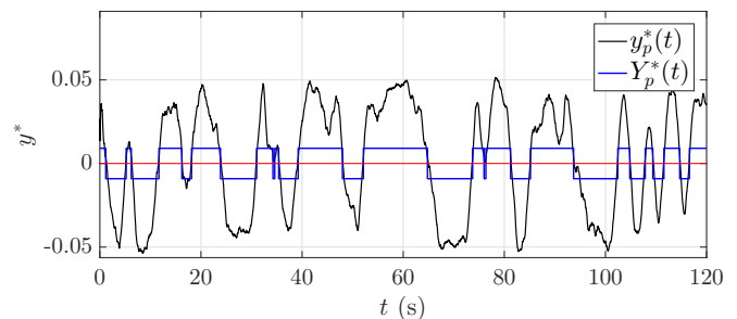
FIG. 15. Part of the telegraph signal Y_p^*(t) (blue) obtained for the pressure barycenter spanwise position y_p^*(t) (black). For clarity the telegraph signal is plotted with a 0.25 factor. Here, y_{C_2}^* = 3.64 \times 10^{-2} \pm 1 \times 10^{-4} .
