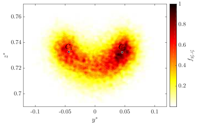
FIG. 9. Normalized two dimensional PDF of the pressure barycenter G_P with the two identified local maxima of the PDF (black squares).
