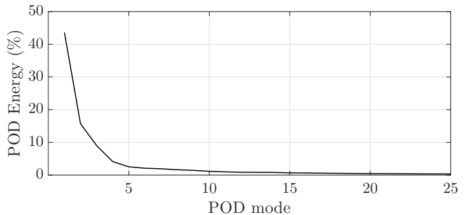
FIG. 6. Energy distribution of the first 25 POD modes of the rear pressure.
