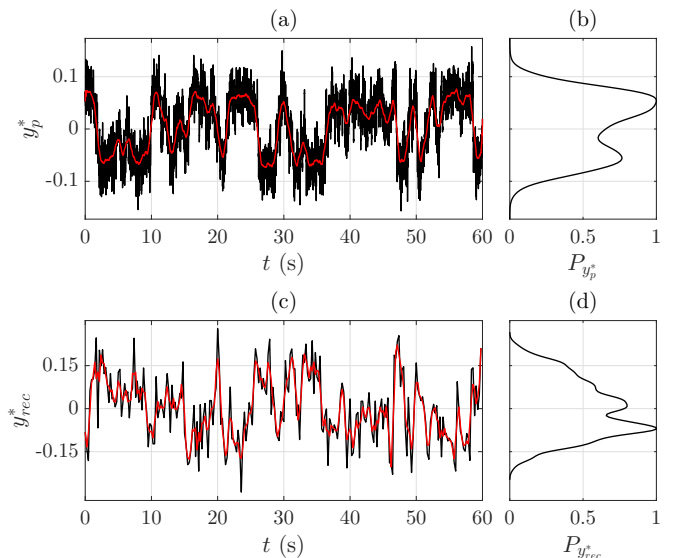
FIG. 3. Pressure barycenter spanwise position y_p^* : (a) evolution in time and (b) normalized PDF P_{y_p^*} for T_P = 1 min ( f_P = 500 Hz). Recirculation intensity barycenter spanwise position y_{rec}^* : (c) evolution in time and (d) normalized PDF P_{y_{rec}^*} for T_{PIV} = 1 min. Red curves show the data smoothed over one second.
