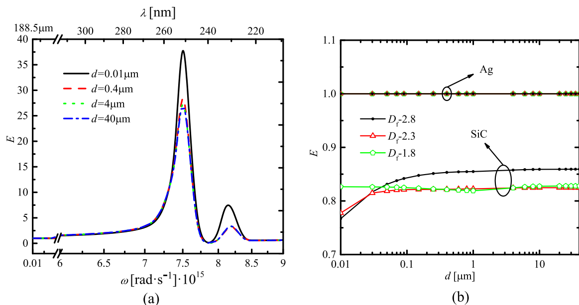
FIG. 6. (a) Enhancement factor of RHT between two Ag nanoparticle clusters with D_f 2.3 for different separation gaps. (b) Enhancement factor of RHT for SiC and Ag nanoparticle clusters as a function of the separating gap.
