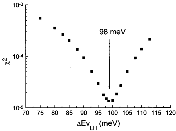
FIG. 3. \chi^2 function vs \Delta E_{v_{LH}} , the valence band discontinuity for light holes. \chi^2 is defined as follows: \chi^2(\Delta E_v) = (\text{ELH1}_{th}^B - \text{ELH1}_{exp}^B)^2 + (\text{ELH1}_{th}^A - \text{ELH1}_{exp}^A)^2 , where \text{ELH1}_{th}^B and \text{ELH1}_{th}^A stand for the theoretical values for the type II transition of samples B (5.3 nm) and A (7.6 nm) and \text{ELH1}_{exp}^B and \text{ELH1}_{exp}^A the experimental data.
