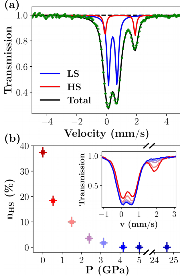
Figure 2: (a) Experimental Mössbauer spectrum obtained for ^{57}\text{Fe}(\text{pyrazine})[\text{Ni}(\text{CN})_4] particles at 0.52 \pm 0.2 GPa and 298 K (green dots). The red and blue solid lines denote the contributions of the HS and LS states, respectively. The fitted curves take into account the thickness effect of the experimental spectrum. (b) Pressure dependence of the HS fraction and the corresponding Mössbauer spectra (inset).
