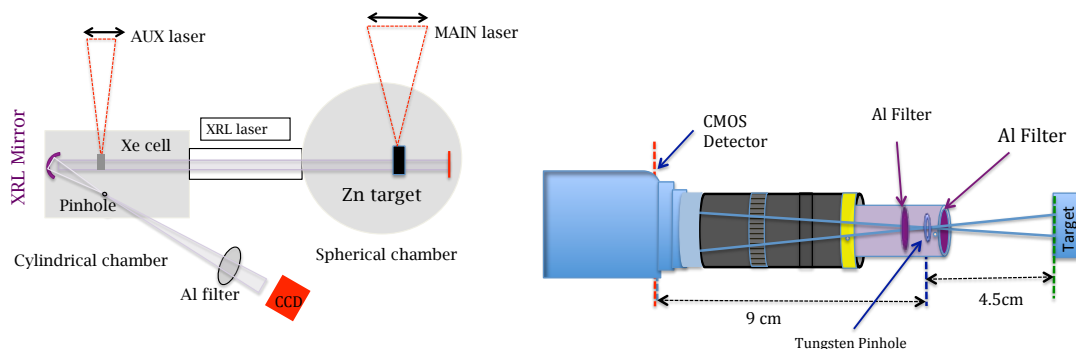
Fig. 1. Left: Schematic experimental set-up. Right: Principle of the keV pinhole imaging system.
