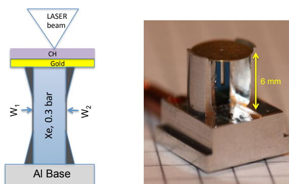
Fig. 2. Left: Target principle; W_1 , and W_2 are two \text{Si}_3\text{N}_4 windows. Right: Image of the target.
