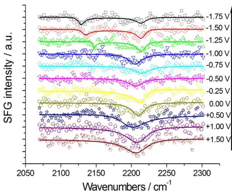
Figure 2. Potential-dependent SFG spectra of Au in contact with [\text{BMP}][\text{TFSA}] containing 1 mM CTDB and the corresponding fits: Cathodic-going scan (from +1.50 V to -1.75 V, starting with pristine Au electrode). The potential scan sequence (cathodic-going scan) is indicated by the arrow.
