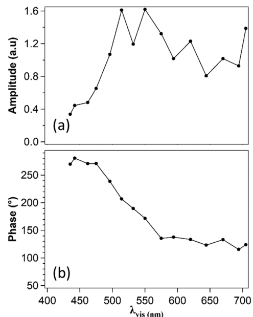
FIG. 6. Amplitude (a) and absolute phase (b) of the effective nonlinear response of gold in the visible range.
