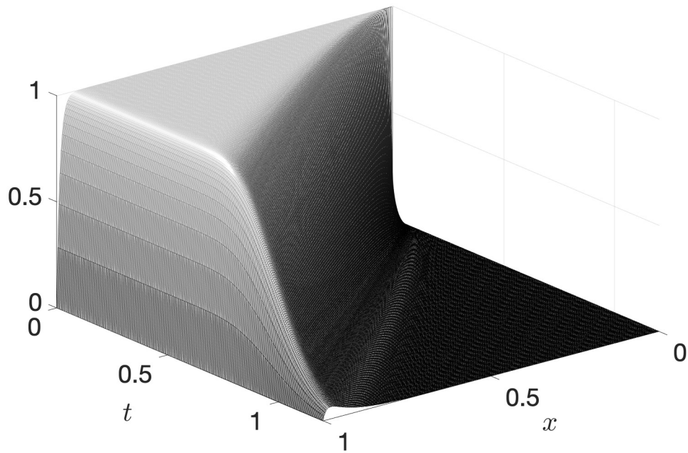
Figure 3: \tilde{P}^\varepsilon(x, t) in (0, 1) \times (0, 1.2/M) ; M = 1 , \varepsilon = 10^{-2} ; v \equiv 0 , y_0 \equiv 1 .
