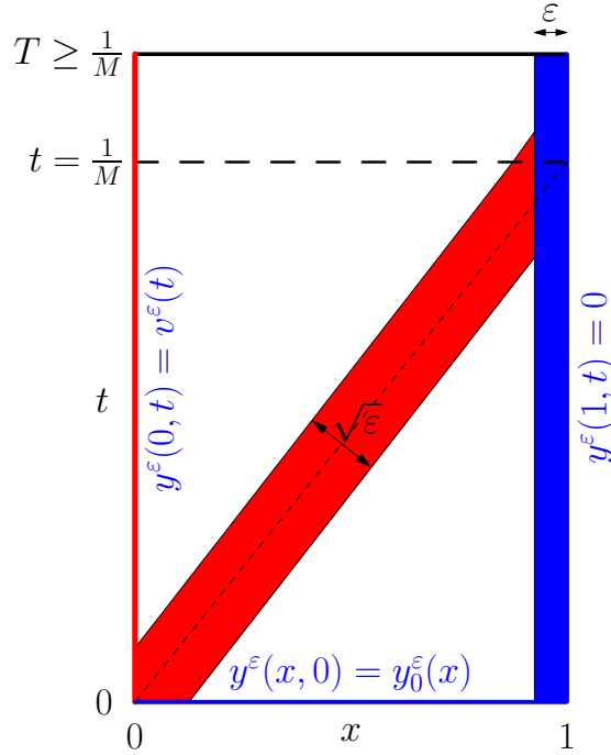
Figure 1: Internal (red) and boundary (blue) layer zones for y^\varepsilon in the case M > 0 .
