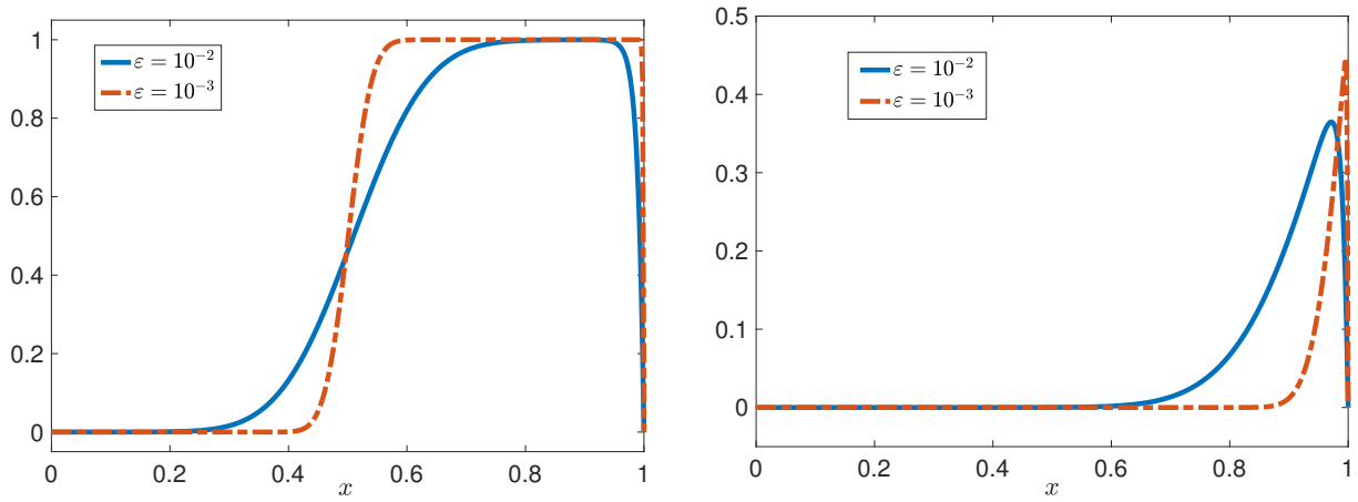
Figure 2: \tilde{P}^\varepsilon(x, t) w.r.t. x \in (0, 1) for t = 1/2/M (left) and t = 1/M (right); M = 1 , \varepsilon \in \{10^{-2}, 10^{-3}\} .
