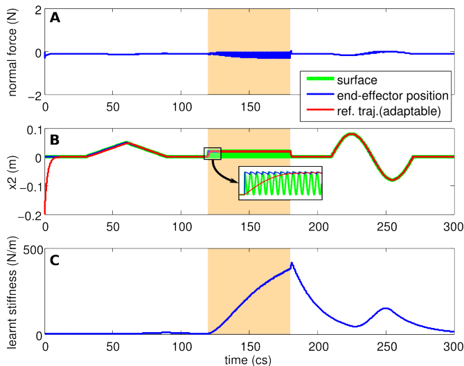
Fig. 4. Surface exploration task simulation: In this task the robot explored an unknown surface and built its map (red trace in B) while moving (blue trace in B). The contact force (along x_2 ) during the movement was maintained (A) at a minimal value while stiffness along x_2 increased (C) only in the presence of a rough texture (orange region) on the surface. The stiffness changes could be thus used to identify the texture of the explored surface.
