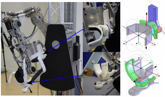
Fig. 11. The two fixations on the exoskeleton
