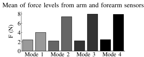
Fig. 7. Mean of force levels for each force/torque sensor (arm and forearm) measured in each mode for the subject 1.
