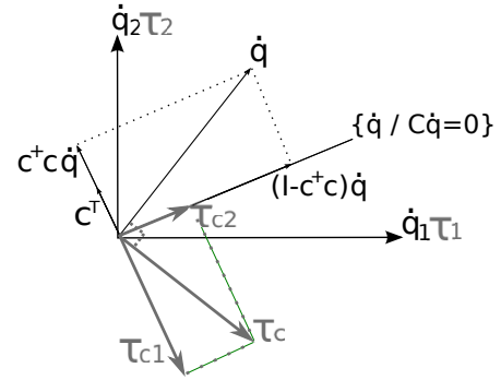
Fig. 1. Representation of the projections in the case of \mathbf{C} = [-1 \ 3] .
