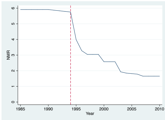
France: NMR
