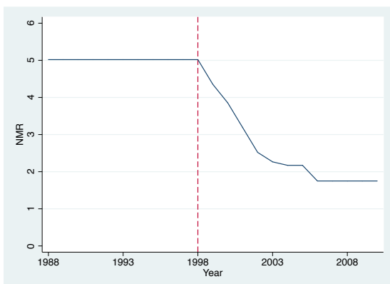
Belgium: NMR
