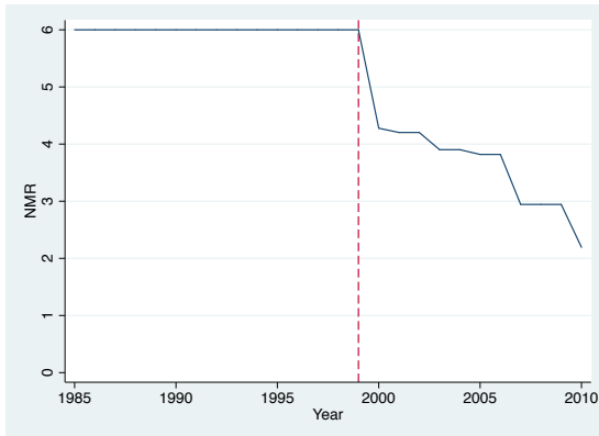
Italy: NMR
