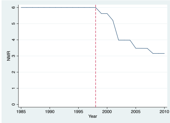
Hungary: NMR
