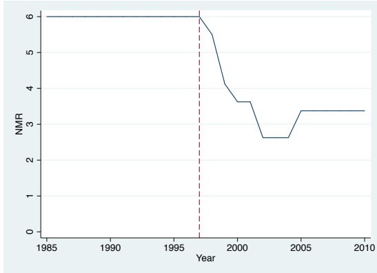
Denmark: NMR
