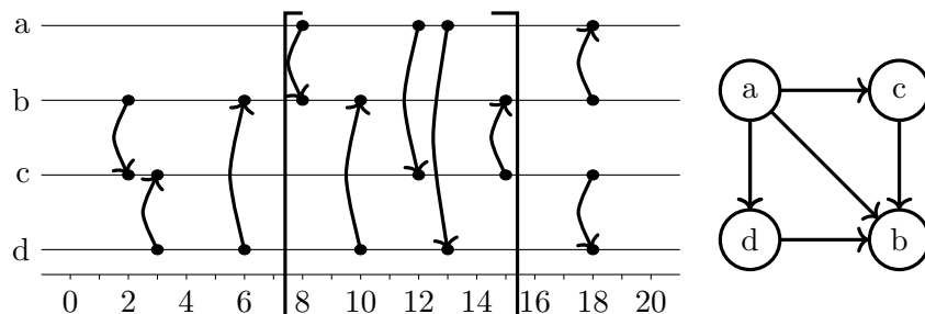
Figure 1: A link stream (left) and its graph projection in time interval [8, 15] (right).
