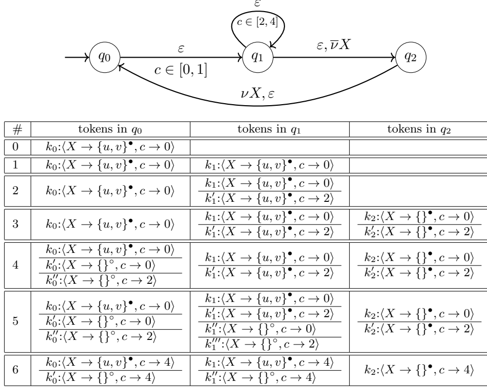
Figure 5: Example of \varepsilon -closure with an input delay 4
