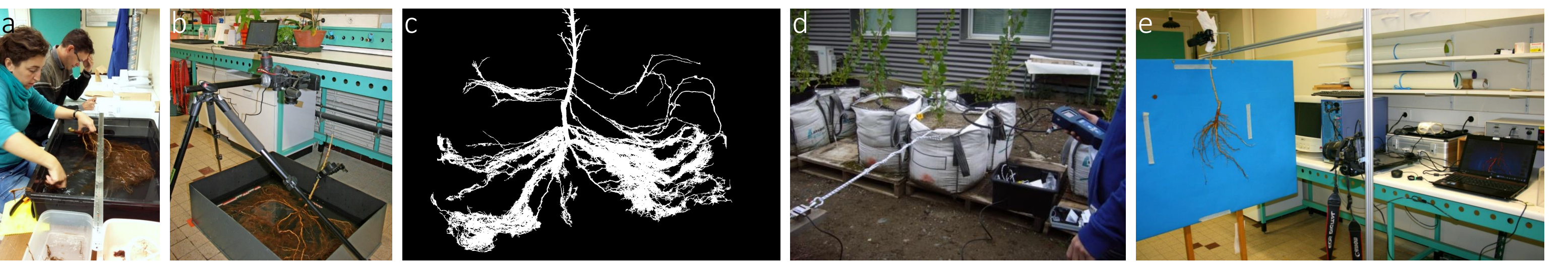
Figure 6. Below-ground trait measurements by hand (a) and from image analysis after the whole-plant extraction (b, c) and after the plant uprooting with a winching device (d, e).
