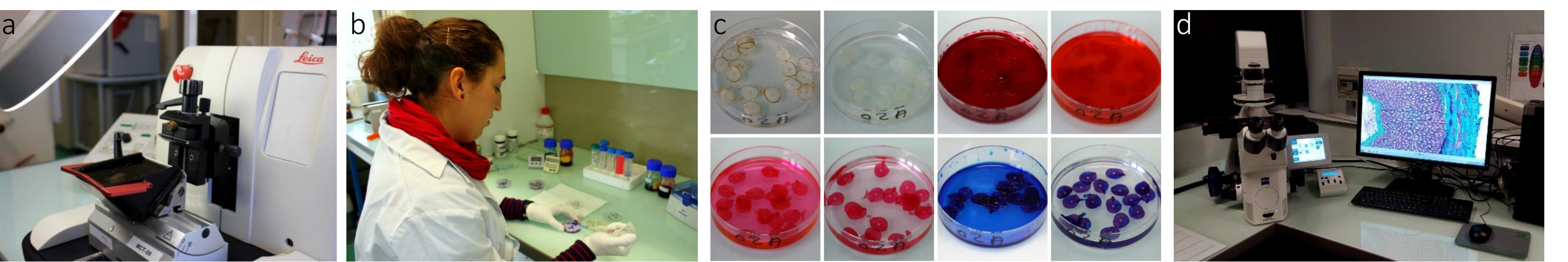
Figure 7. Preparation of anatomy sections (a-c) and image processing (d) for anatomical trait measurements.
