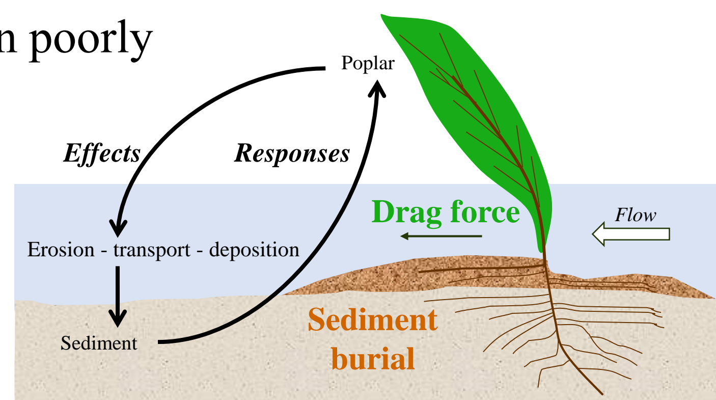
Figure 1. Reciprocal interaction between vegetation and water and sediment dynamics.
