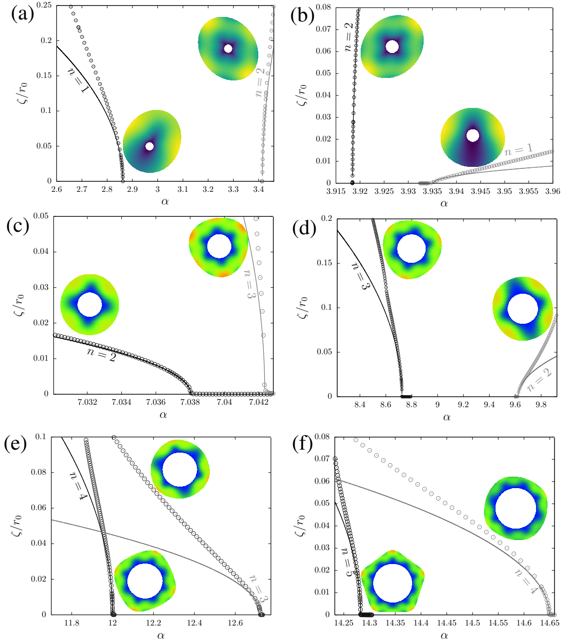
FIG. 9: Amplitudes \zeta of modes of deformation as a function of the load parameter \alpha , for different relative radius of the inner cylinder (values of a are 0.15, 0.22, 0.42, 0.5, 0.6, 0.65 in figs (a), (b), (c), (d), (e) and (f) respectively). Solid lines are for amplitudes computed from the analytic expression Eq.29. Empty circles and the snapshots originate from finite element simulations of Section V. The amplitude of the unstable mode with the lowest value of \alpha_c is in black (circumferential wave numbers are respectively n_{\text{first}} = 1, 2, 2, 3, 4 and 5 ), and the amplitude of the second mode with the lowest value of \alpha_c is in gray (circumferential wave numbers are respectively n = 2, 1, 3, 2, 3 and 4 ). The other modes are not shown in these figures. Deformed shapes obtained by simulations are shown in the insets ; the color map represents the magnitude of the displacement increasing from blue (no displacement) to orange.
