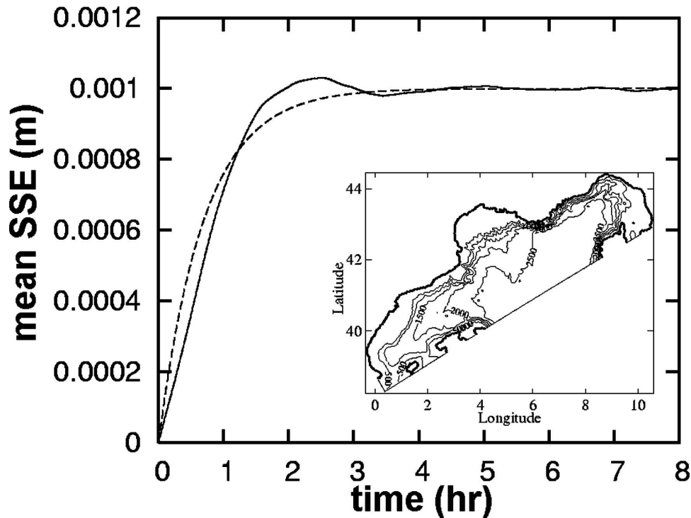
FIG. 2. Mean sea surface elevation computed during an 8-h barotropic run initialized at rest and forced at open boundaries by a sea surface elevation of 0.001 m and zero current (solid line), and corresponding analytical solution computed from Eq. (19) using a domain-averaged value of the barotropic wave celerity (dotted line). The insert presents the domain modeled in the northwestern Mediterranean.
