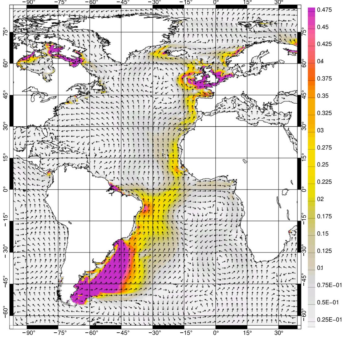
Fig. 6. Spectral energy flux associated with the propagation of the M_4 tide in the ocean ( \text{W m}^{-1} ). This term is computed for a T-UGOm 2D global ocean simulation forced with the astronomic potential and the loading and self-attraction effects of the major astronomical tides. The computational mesh is the one used in FES2004 with a Lagrange-P1 approximation.
