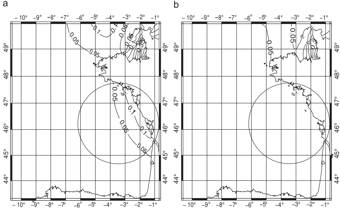
Fig. 10. Influence of M_4 initialization and barotropic forcing at the boundaries over the amplitude of the surface elevation modeled with SYMPHONIE. (a) Amplitude for M_4 solution (m) in the case of initialization and boundary forcing using T-UGOm solutions and (b) amplitude (m) for M_4 solution in the case without forcing at the boundaries. The circle indicates the region where the forcing has the stronger impact.
