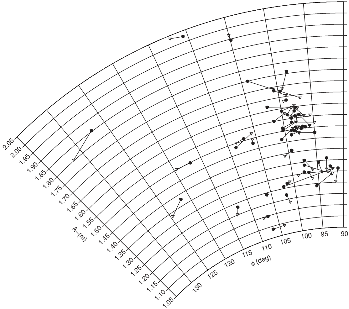
Fig. 11. Polar plot (amplitude and phase) of the comparison of the tidal component M_2 between the SYMPHONIE solution (empty triangles) and the solution from the tide gauges (full circles).
