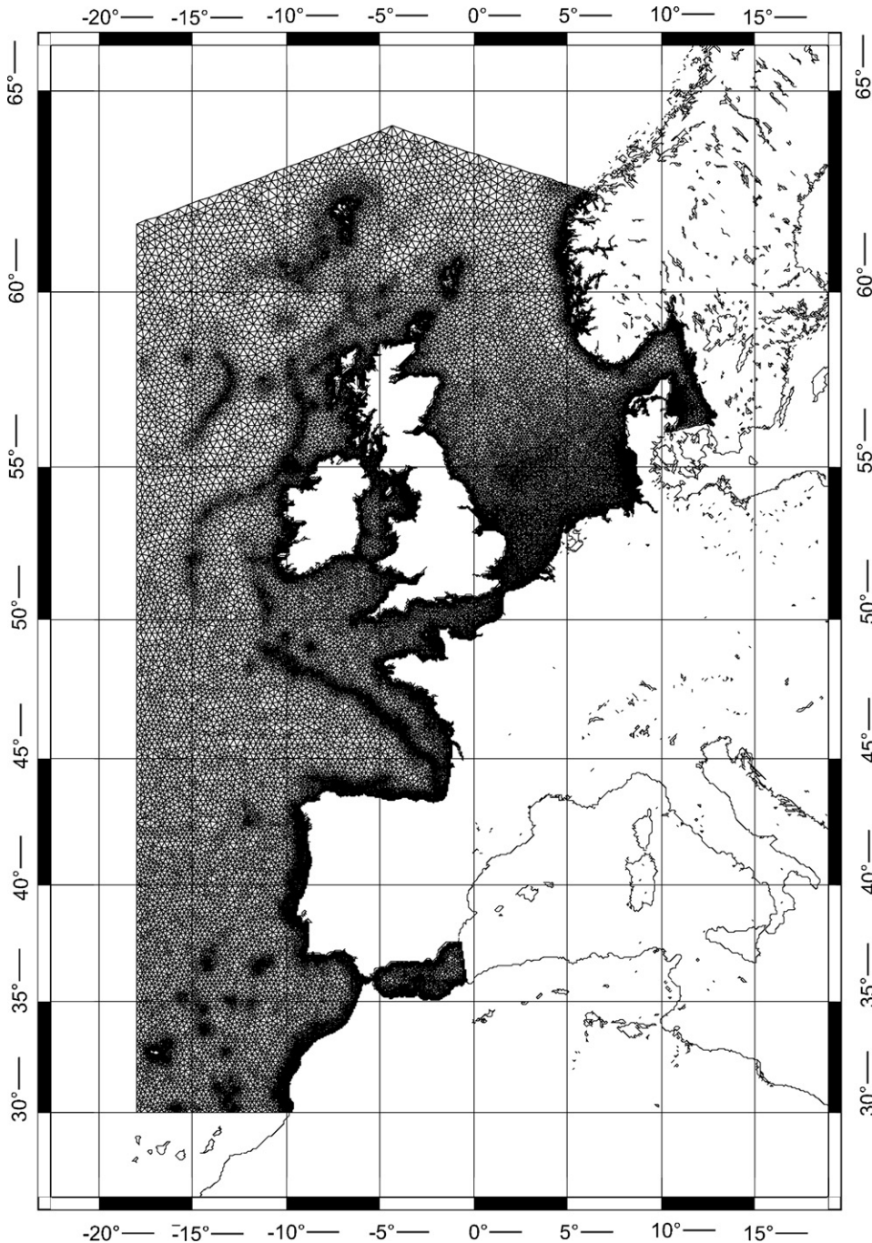
Fig. 1. NEA-2004 finite-element mesh.
