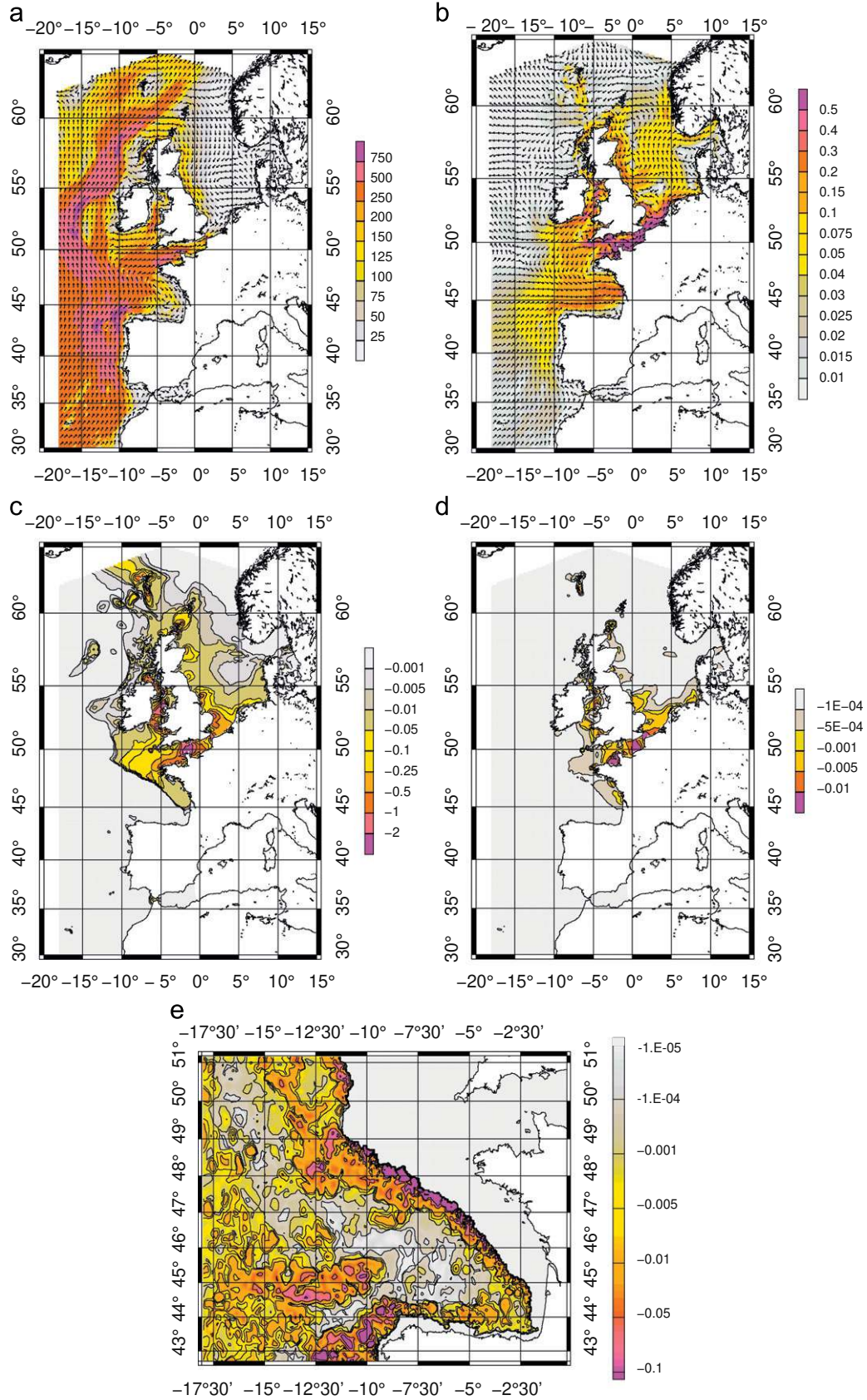
Fig. 7. Spectral energy flux (a and b), bottom friction (c and d) and wave drag (e) dissipation rate of work for the M_2 (a, c and e) and M_4 (b and d) tides. Units are \text{W m}^{-1} for the fluxes and \text{W m}^{-2} for the rate of work.
