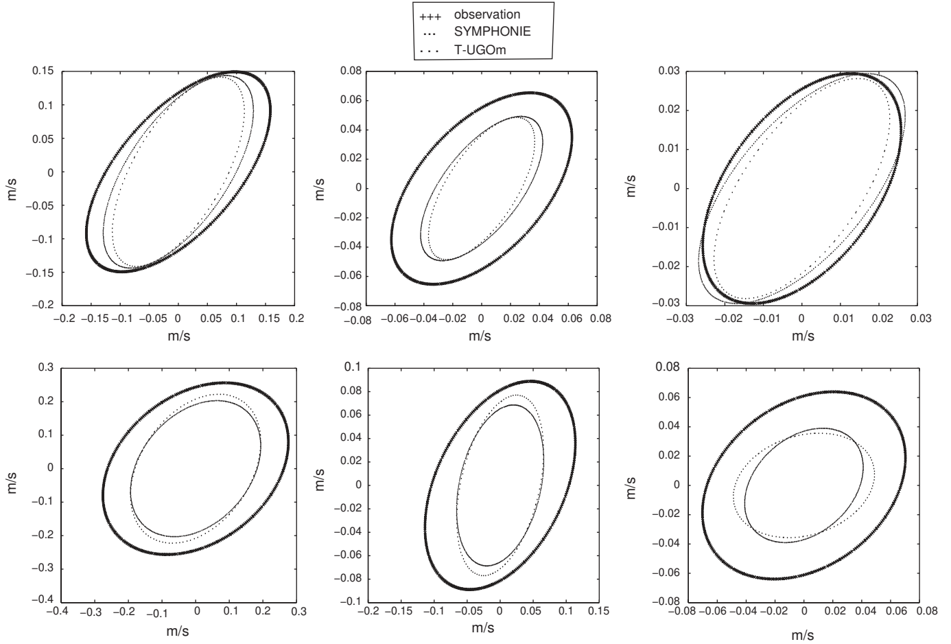
Fig. 12. Comparison of current ellipses for SYMPHONIE and T-UGOm interpolated solutions and observations at locations DP94-1 (upper row) and DP94-2 (lower row) (Perenne and Pichon, 1999; Pichon and Correard, 2006) for M_2 , S_2 and N_2 waves (in this order from left to right).
