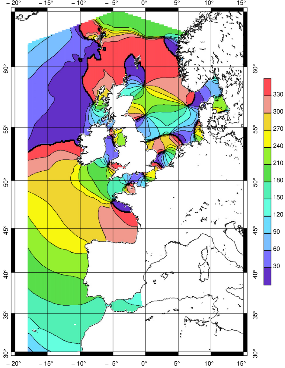
Fig. 5. Phase lag of the M_4 tide computed from T-UGOm 2D. Units in degrees.
