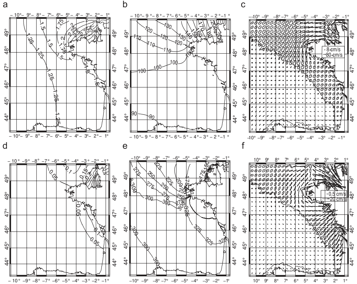
Fig. 9. Characteristics for the semi-diurnal M_2 and quarter-diurnal M_4 barotropic tides. Maps after a harmonic analysis performed over two months for a barotropic SYMPHONIE simulation with a forcing by M_2 , S_2 , N_2 , K_1 and M_4 : (a) M_2 tidal surface elevation amplitude (m), (b) M_2 tidal surface elevation phase lag (deg), (c) M_2 tidal current ellipses ( \text{cm s}^{-1} ), (d) M_4 tidal surface elevation amplitude (m), (e) M_4 tidal surface elevation phase lag (deg) and (f) M_4 tidal current ellipses ( \text{cm s}^{-1} ).
