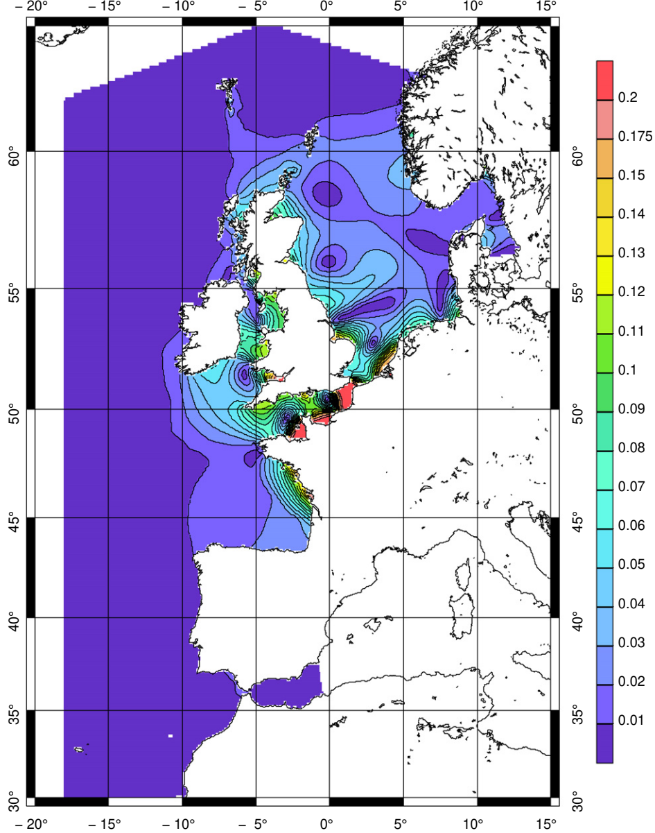
Fig. 4. Amplitude of the M_4 tide computed from T-UGOm 2D. Units in meters.
