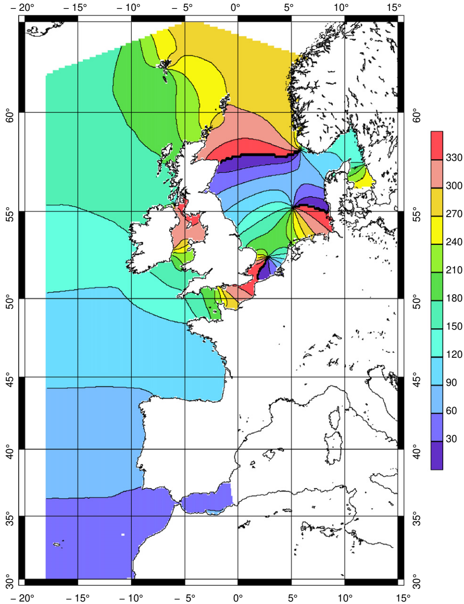
Fig. 3. Phase lag of the M_2 tide computed from T-UGOm 2D. Units in degrees.
