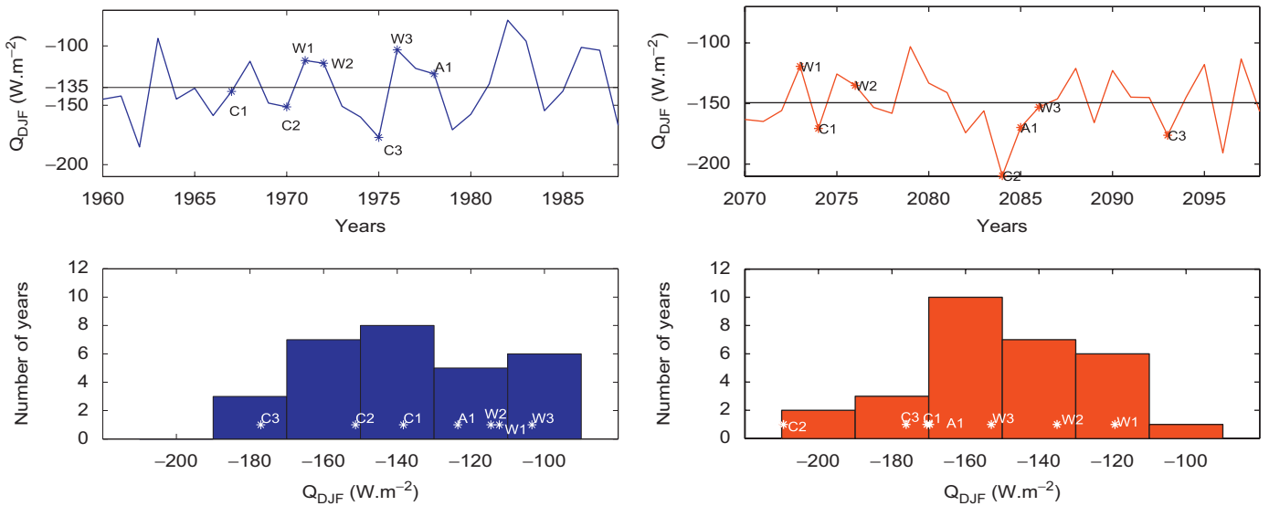
Fig. 1. Selection of representative years in the present (left) and future (right) periods. Top: winter heat flux averaged over the NWMS in the ARCM simulation, Q_{DJF} = -HL_{DJF} . The black line corresponds to the winter heat loss averaged over the whole period. Bottom: distribution of Q_{DJF} in the ARCM simulation. Value of Q_{DJF} for each selected year is marked by an asterisk and the corresponding year name.
