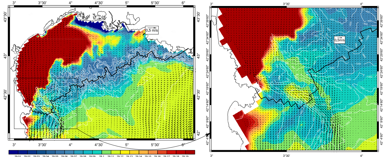
Fig. 6. Cascading event on 25th February of year C2 of the present period ( \rho_{crit} = 29.105 kg m^{-3} ). Bottom density ( kg m^{-3} , map) and current ( m s^{-1} , arrows). White lines: topography. Black line: SDS boundary.
