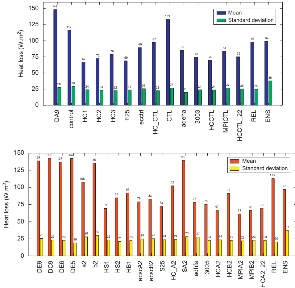
Fig. 11. Average and standard deviation of the mean December–March total heat loss over NWMS, HL_{DJFM} ( W m^{-2} ), for each present-day climate simulation (top) and end of the XXIth century simulation (bottom) selected from the PRUDENCE project. REL corresponds to the heat loss of the ARCM ARPEGE-Climate simulations DA9 and DE9 corrected by the relaxation term, used to force the regional model SYMPHONIE (see Section 2.1). ENS corresponds to the 240-year ensemble mean formed by the eight present-day climate simulations for the eight ARCM (see Tables 5 and 6).
