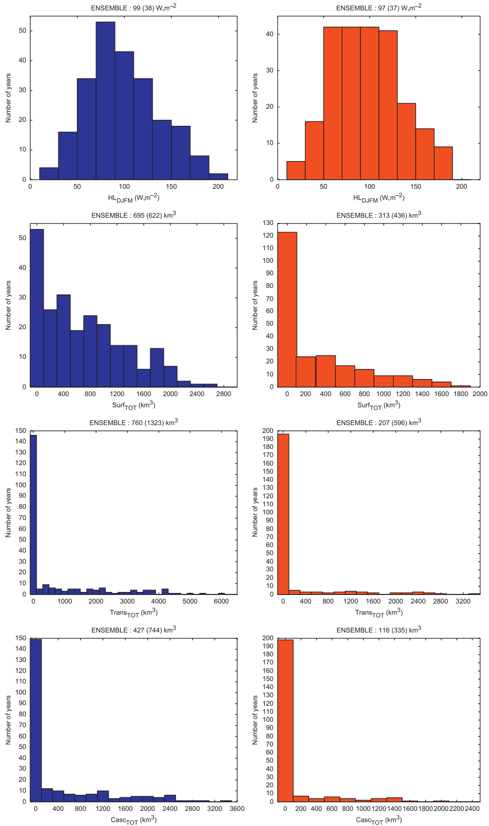
Fig. 14. Distribution of the heat loss HL_{DJFM} ( W \cdot m^{-2} ) and of the DW formed at the surface Surf_{TOT} , exported Trans_{TOT} , and cascading Casc_{TOT} for the mean ensemble ENS ( km^3 ) under present-day climate conditions (left) and at the end of the XXIth century (right). The average and standard deviation are indicated.
