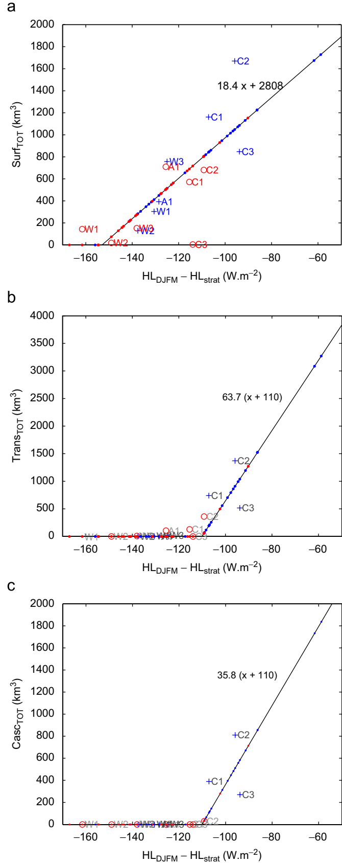
Fig. 9. DW formed, exported and cascading for the present (blue) and future (red) periods. (a) Total DW volume formed at the surface during a given year, Surf_{TOT} , as a function of the difference between the mean heat loss during the formation period for this given year and the mean heat loss corresponding to the stratification, HL_{DJFM} - HL_{strat} . (b) and (c) Same for exported water Trans_{TOT} and cascading water Casc_{TOT} . + and o: selected years for the present and future periods. •: results obtained for each year of the present and future period using the obtained regression. Black line: linear regression analysis.
