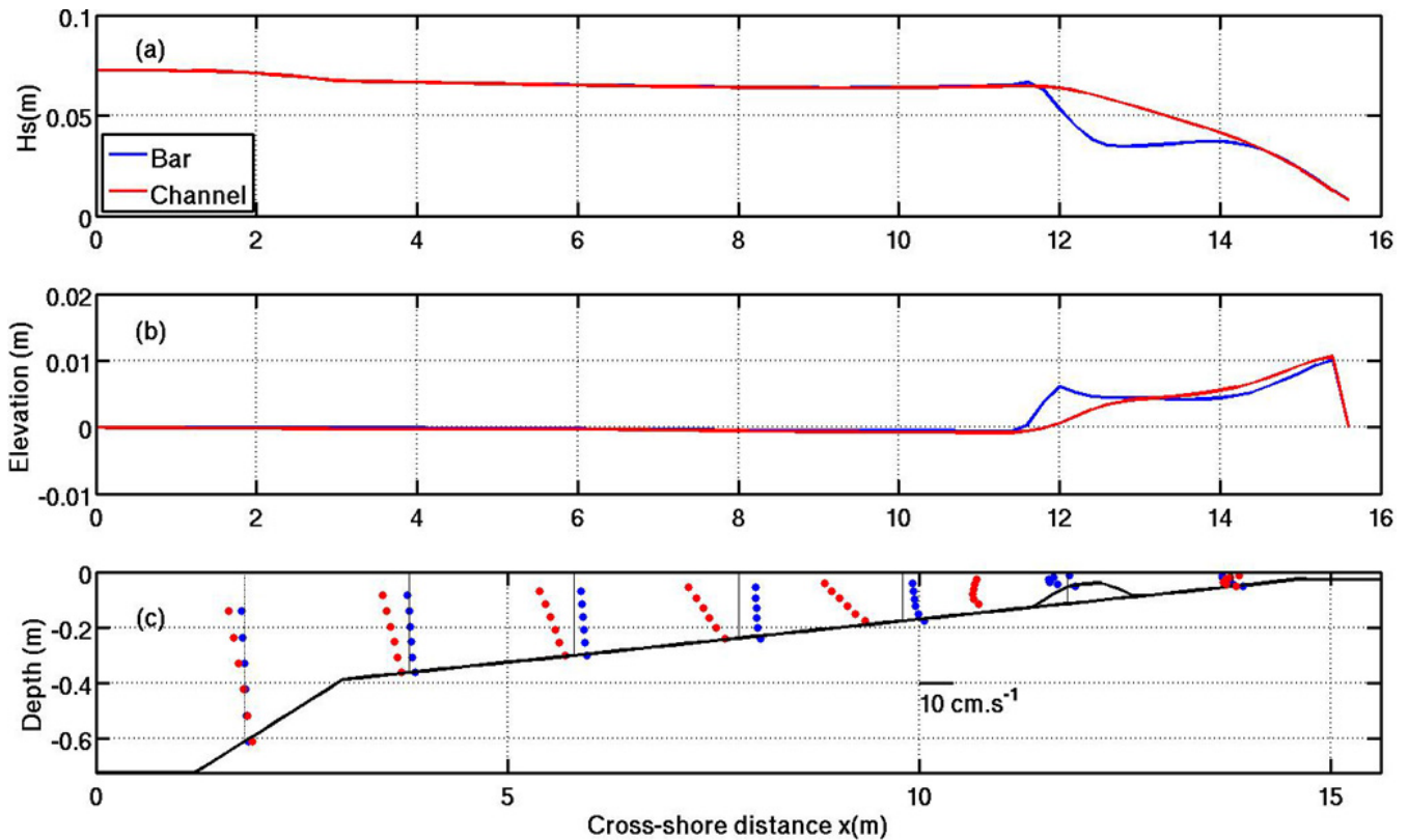
Fig. 5. Significant wave height (a), surface elevation (b) and vertical profiles of the cross-shore velocities (c) versus cross-shore distance over the center bar at y = 9.2 m (blue) and through the rip channel at y = 4.6 m (red). The shoreline is at right.
