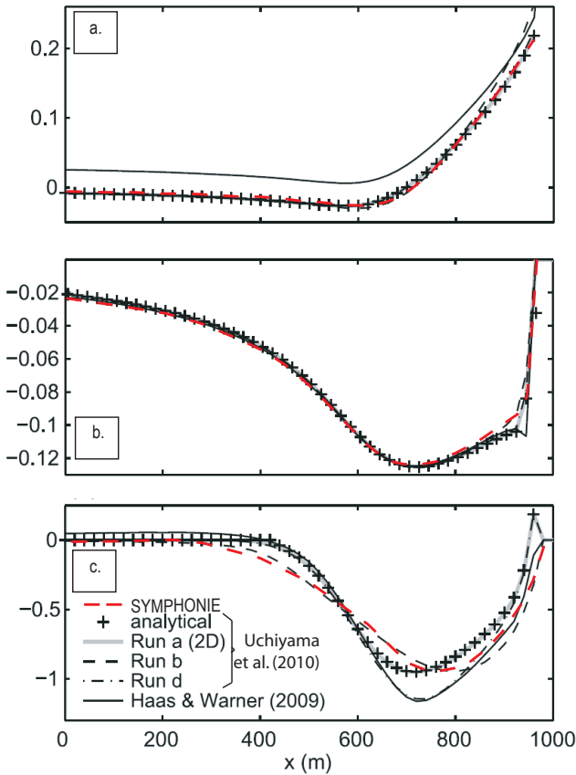
Fig. 1. Cross-shore profile of the surface elevation (a), barotropic quasi-Eulerian cross-shore (b) and longshore (c) velocities ( \text{m s}^{-1} ) (adapted from UMS10). SYMPHONIE results are the red dashed line whereas ROMS results of Run b are in black dashed lines. The shoreline is at right.
