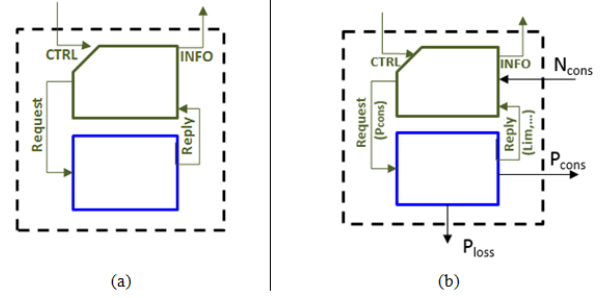
Figure 4. Representations of (a) generic and (b) source elements.
