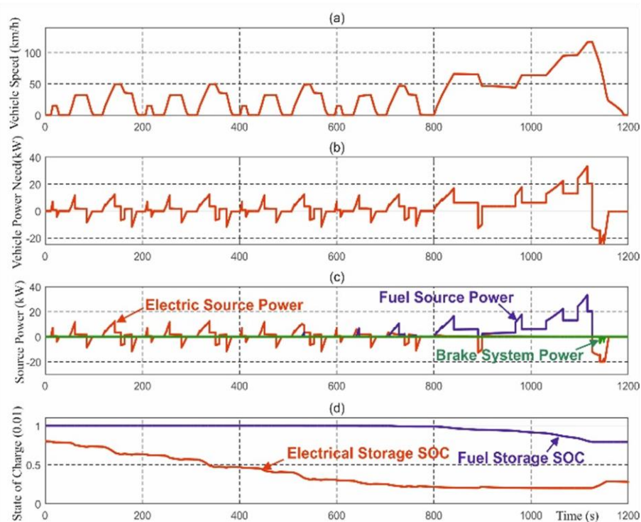
Figure 11. Functional model simulation of a parallel HEV.
