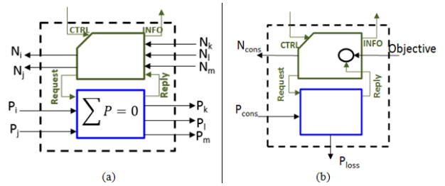
Figure 6. Representations of (a) distribution and (b) effector elements.
