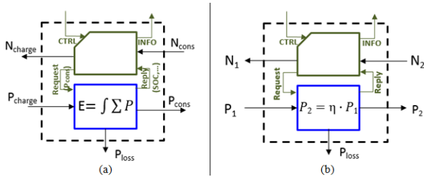
Figure 5. Representations of (a) storage and (b) transformation elements.
