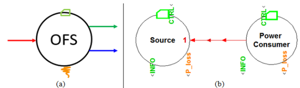
Figure 7. (a) Representation of OFS and (b) example PhiSim link.
