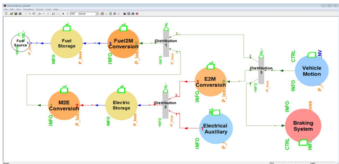
Figure 8. PhiSim functional model of a parallel HEV.
