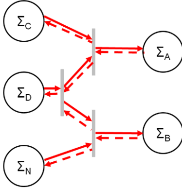
Figure 3. A system example with multiple source and consumer ports.
