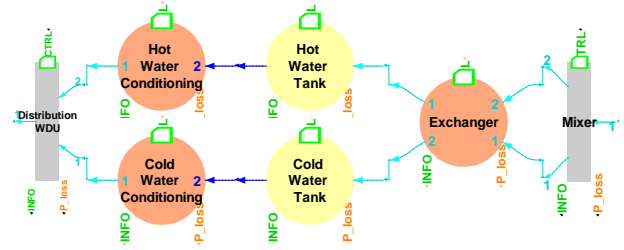
Figure 10. Waste water distribution unit functional model.
