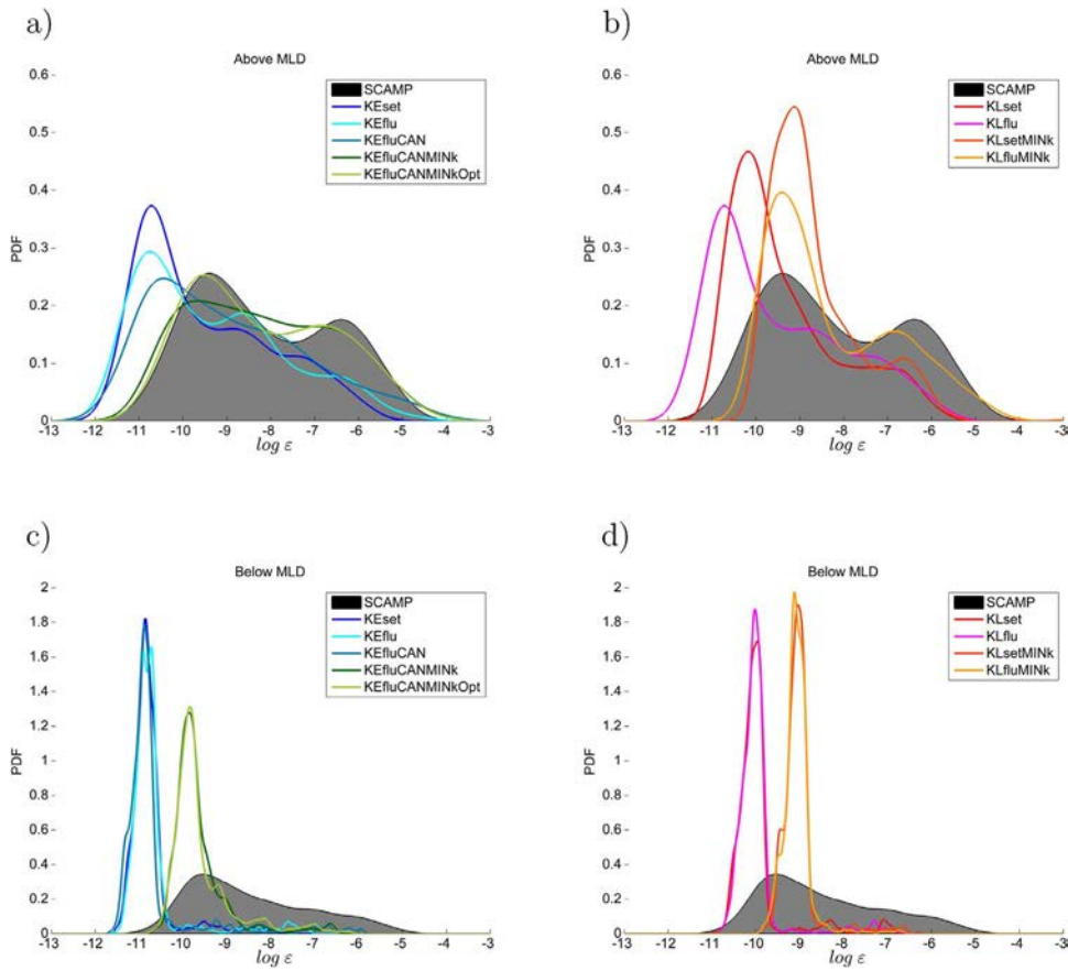
Fig. 5. a) and b): \epsilon probability density functions issued from all the in situ (black shade) and numerical data (thick lines) in the surface mixed layer for the KE closure scheme and the KL closure scheme respectively. c) and d): the same but below the surface mixed layer.
