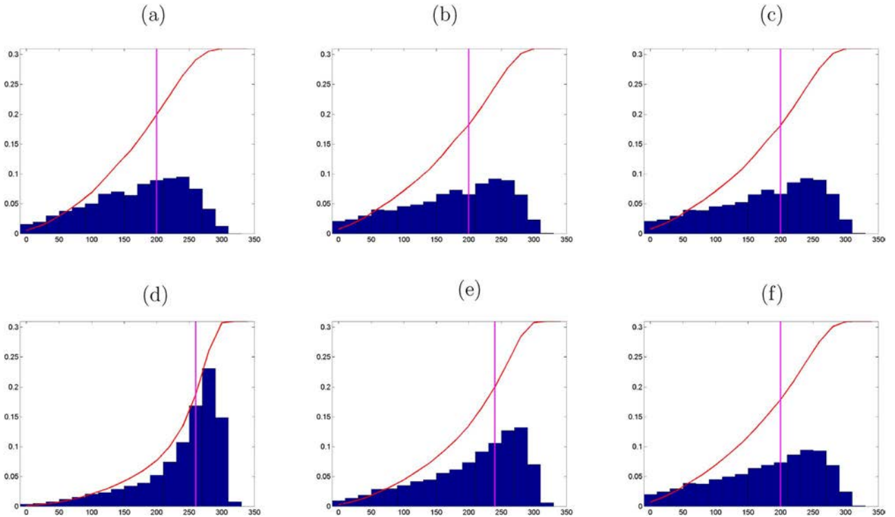
Fig. 9. a) JP values distribution obtained with the II91 segmentation method, b) same as a) for S11, c) same as a) for C12, d) same as a) for M12. e) same as a) for a constant 512 points segmentation. f) same as a) for a 1024 points segmentation with 30% overlap. The red curve is the cumulative distribution of JP values for each case and the vertical line marks the point where the cumulative distribution equals 0.6. The database for this analysis comprehended 126 profiles with an average depth of 50 m in various meteorological conditions in the Gulf of Lion. (For interpretation of the references to color in this figure legend, the reader is referred to the web version of this article.)
