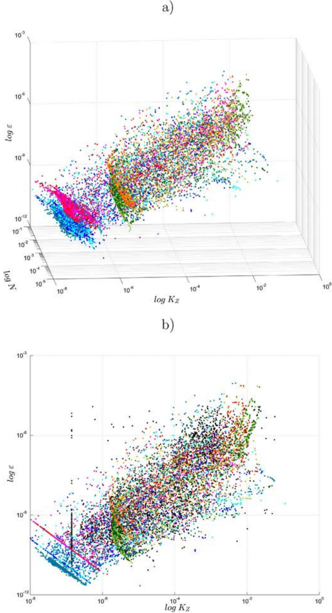
Fig. 8. a) All in situ (in black) and numerical data of K_z , N and \varepsilon . b) All in situ (in black) and numerical data of K_z and \varepsilon . The color code is the same as in the other figures.
