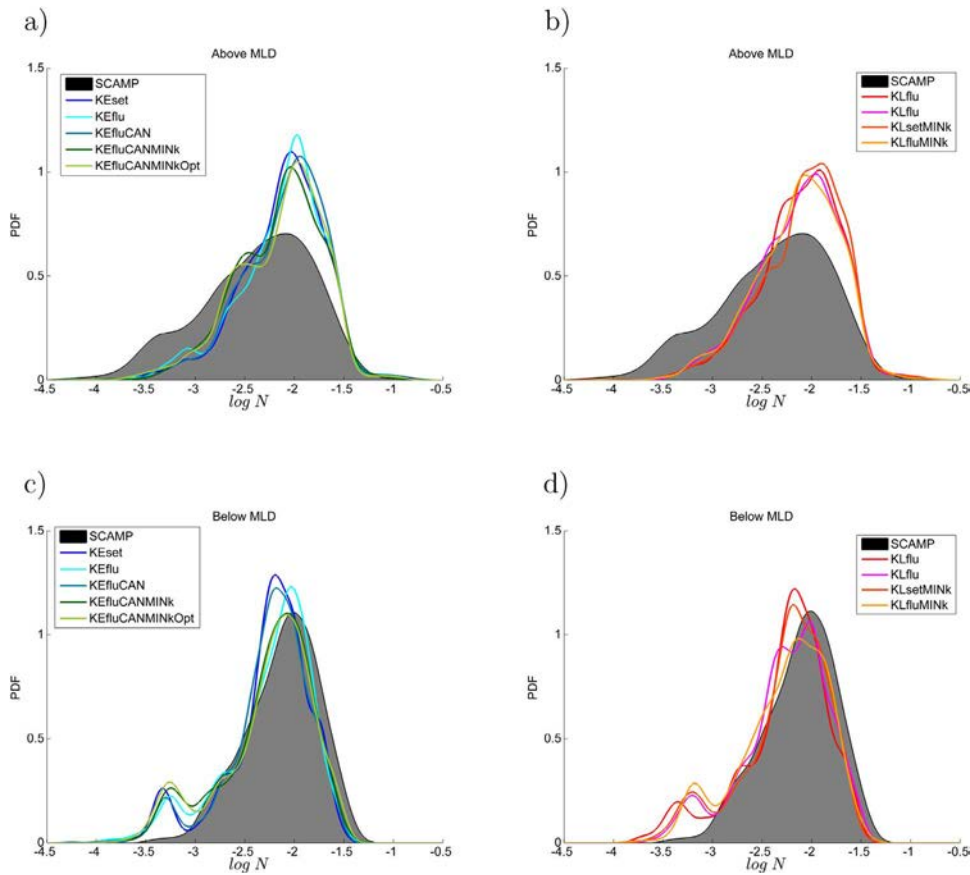
Fig. 6. a) and b): N probability density functions issued from all the in situ (black shade) and numerical data (thick lines) in the surface mixed layer for the KE closure scheme and the KL closure scheme respectively. c) and d): the same but below the surface mixed layer.
