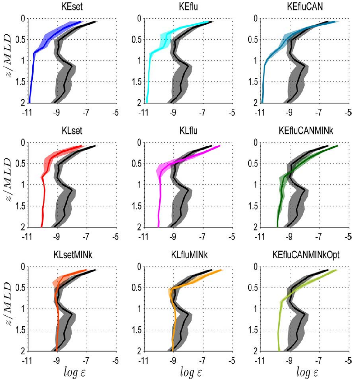
Fig. 2. The thick lines represent median values of \varepsilon estimated from in situ data (in black) and numerical experiments. The shades indicate 95% bootstrap confidence intervals. Water depth z is non-dimensionalised with respect to the mixed layer depth MLD for each profile.
