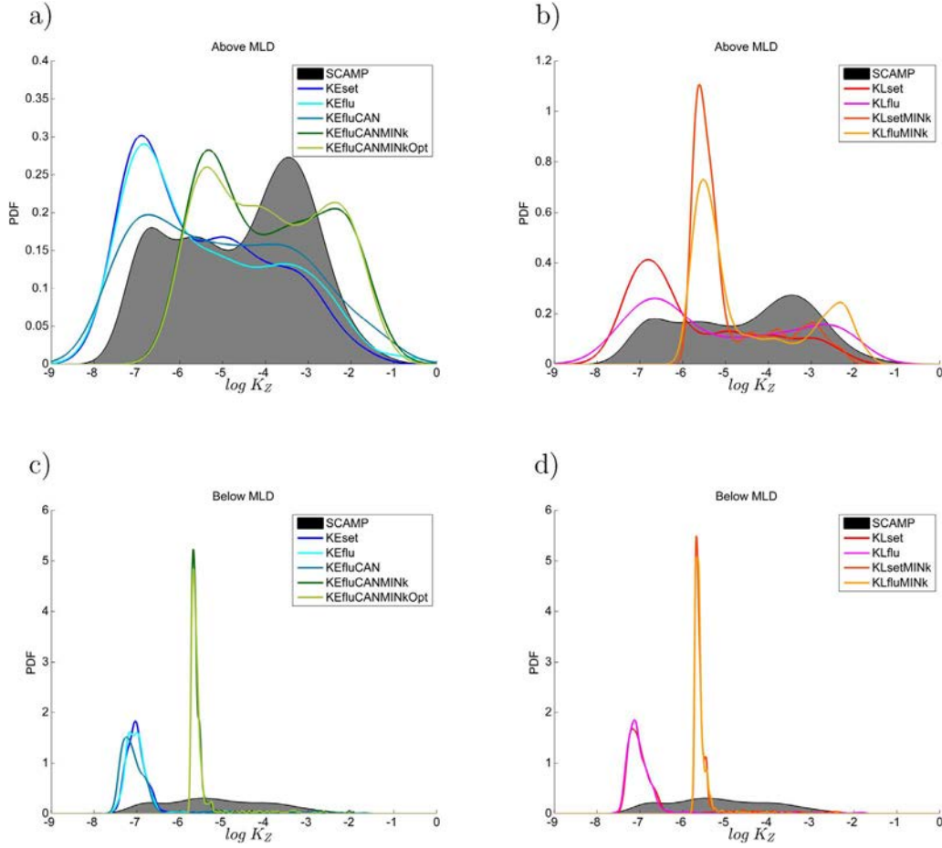
Fig. 7. a) and b): K_Z probability density functions issued from all the in situ (black shade) and numerical layer data (thick lines) in the surface mixed layer for the KE closure scheme and the KL closure scheme respectively. c) and d): the same but below the surface mixed layer. Note the difference in the range of the y axes in a) and b).
