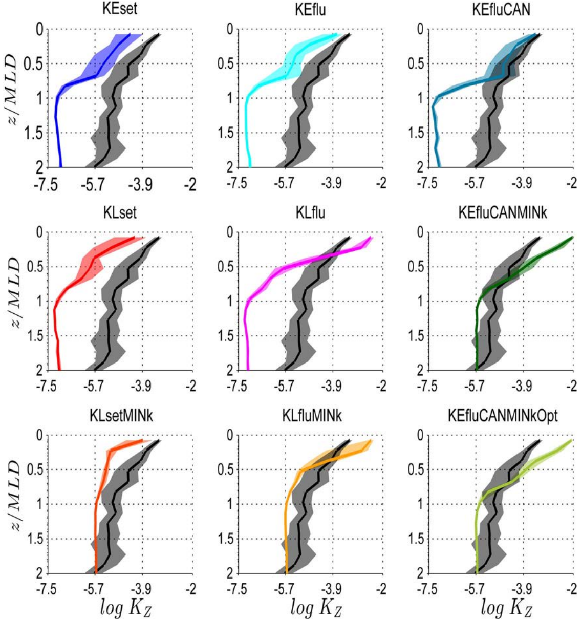
Fig. 4. The thick lines represent median values of K_Z estimated from in situ data (in black) and numerical experiments. The shades indicate 95% bootstrap confidence intervals. Water depth z is non-dimensionalised with respect to the mixed layer depth MLD for each profile.
