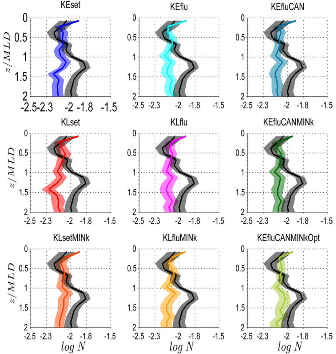
Fig. 3. The thick lines represent median values of N estimated from in situ data (in black) and numerical experiments. The shades indicate 95% bootstrap confidence intervals. Water depth z is non-dimensionalised with respect to the mixed layer depth MLD for each profile.
