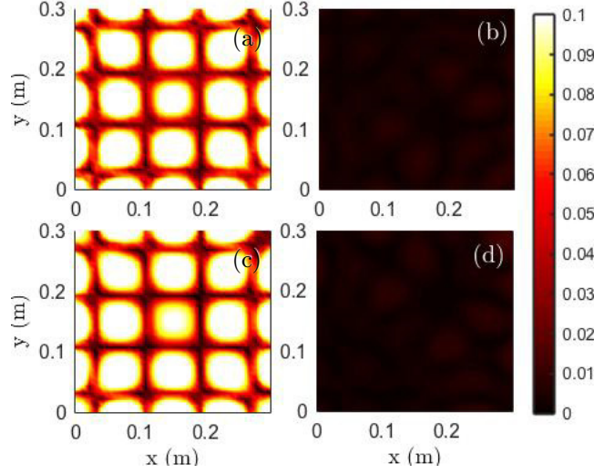
Figure 6: (Color online) Mobility profiles ( \text{m.s}^{-1}/\text{N} ) for the mode A. (a) Theoretical, (c) experimental uncontrolled. (b) Theoretical, (d) experimental controlled.
