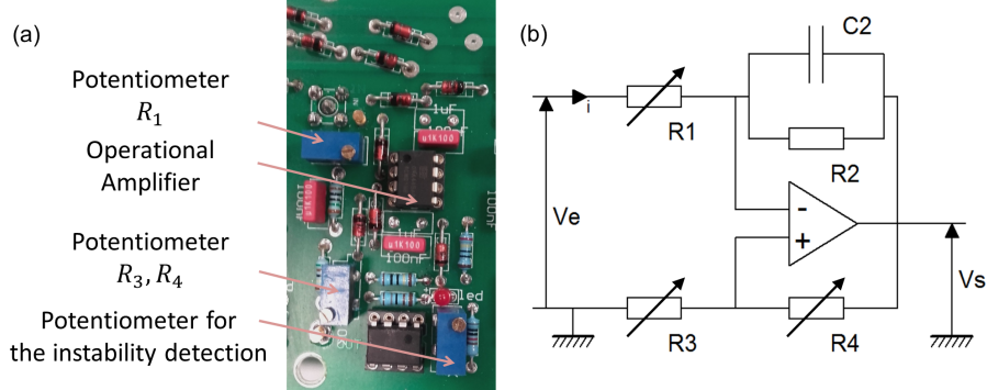
Figure B.7: (Color online) Picture (a) and schematic representation (b) of the analogical electrical circuit of the negative capacitance synthesis.
