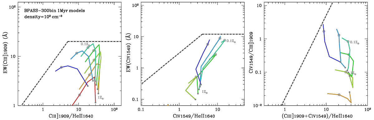
Fig. 4. As in Fig. 2, but for the SED of BPASS binary star models, BPASS-300bin (cyan dotted curve in Fig. 1a). Only the metallicity range of Z = 0.05\text{--}1Z_{\odot} is considered.
