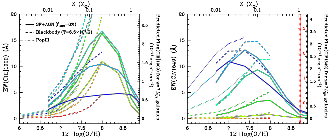
Fig. 18. As in Fig. 13, but with models of mixed SF+AGN ( f_{AGN} = 8\% , solid), blackbody ( T = 6.5 \times 10^4 \text{ K} below Z = 0.2 Z_{\odot} , dashed), and PopIII star (below Z = 0.05 Z_{\odot} , dotted). In each plot, the right ordinate presents a flux predicted for L_{UV}^* galaxies at z = 7 with an EW corresponding to the left ordinate. For the CIV emission, the red right ordinate is added which shows a predicted flux if the stellar CIV absorption exists with EW_{abs}(CIV) = -3 \text{ \AA} .
