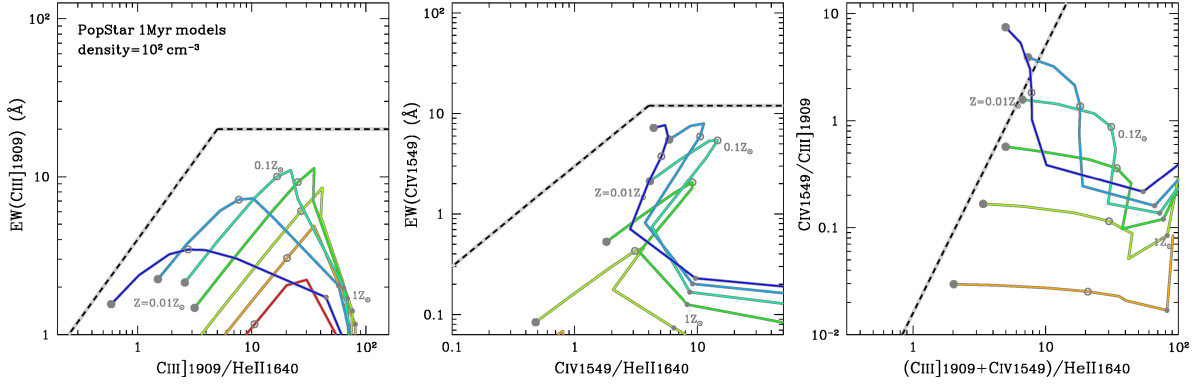
Fig. 2. UV line diagrams for the SED of POPSTAR models (Fig. 1a). A gas density of 10^2 \text{ cm}^{-3} is assumed. The curves present our grid of models in the range of Z = 0.01\text{--}2Z_{\odot} for \log U = -3.5 (red), -3.0 (orange), -2.5 (yellow), -2.0 (green), -1.5 (cyan), -1.0 (skyblue), and -0.5 (blue). The metallicity of Z = 0.01, 0.1 , and 1Z_{\odot} is denoted with a large filled, medium open, and small gray-filled circle, respectively, along each of the curves. The black dashed curves are the demarcations between a star-forming galaxy and AGN that will be defined in Sect. 4.1.
