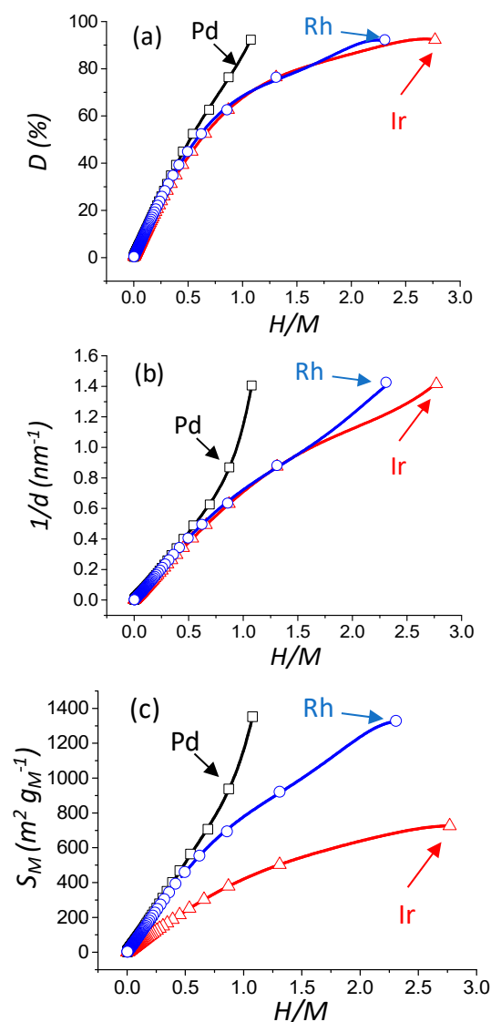
Figure 3. Evolution of the theoretical dispersion versus H/M theoretical ratio ( M = Pd, Ir, \text{ or } Rh ) (a). Evolution of the theoretical reciprocal particle size versus H/M theoretical ratio (b). Evolution of the theoretical metallic specific surface area versus H/M theoretical ratio (c). Open square, triangle, and circle: result of the statistical model calculation of this work for Pd, Ir, and Rh, respectively. The black, blue, and red curves are the fitting result ( R^2 = 1.000 ) with a 5th order polynomial trend line (see Equations (8)–(10)) for Pd, Rh, and Ir, respectively.
