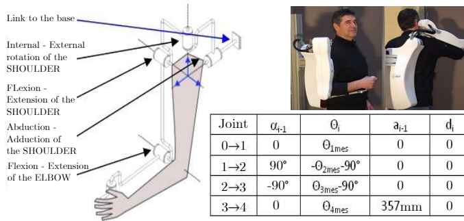
Fig. 9. Kinematics of ABLE
