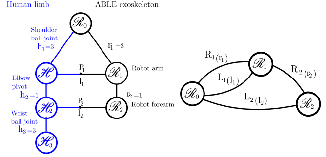
Fig. 10. Schematic of ABLE and human arm coupling
