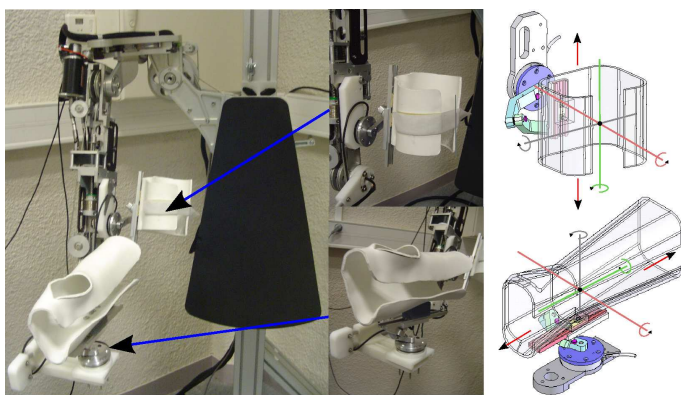
Fig. 14. The two fixations on the exoskeleton
