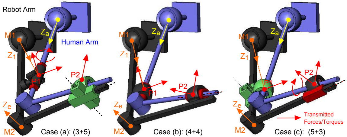
Fig. 11. Three options for coupling ABLÉ to a human arm. Case (a): the 3 DoF upper arm fixation mechanism combines one universal joint and one slider while the 5 DoF lower arm fixation mechanism includes one ball joint and two sliders; case (b): both the 4 DoF fixation mechanisms combine one ball joint and one slider; case (c): symmetrically to case (a), the 5 DoF upper arm fixation mechanism combines one ball joint and two sliders while the 3 DoF lower arm fixation mechanism includes one universal joint and one slider. Arrows in red represent the forces and moments that can be transmitted through the passive fixations, which are complementary to the passive DoF.
