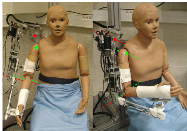
Fig. 15. A manikin connected to ABLE: the shoulder centers and the elbow axes are significantly mismatched
