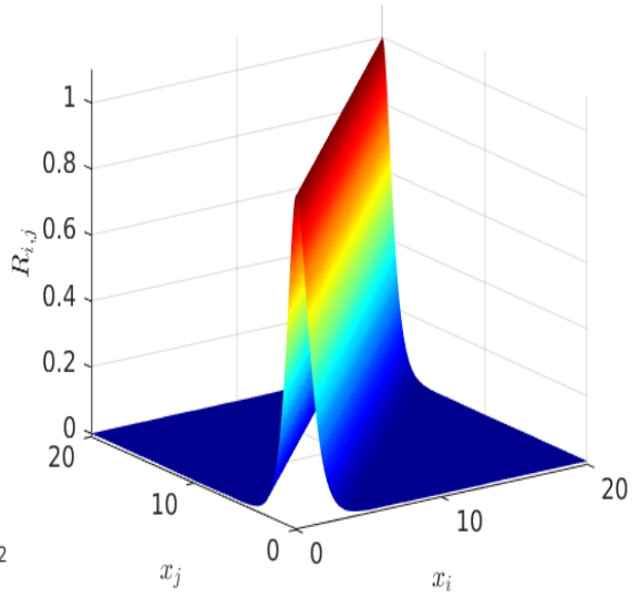
Figure 4: Covariance matrix with MC sampling, \nu = 2 , N = 400 and L = 20
