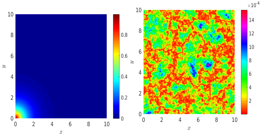
Figure 13: Absolute error |C - C_N| with MC sampling
