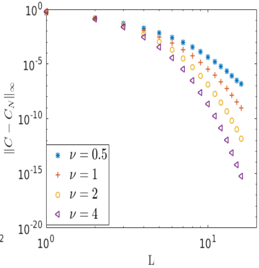
Figure 6: \|C - C_N\|_\infty with respect to L .
