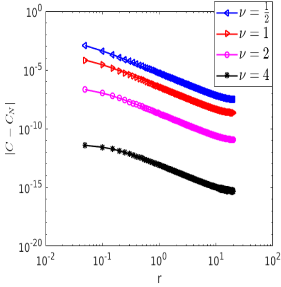
Figure 3: absolute error |C - C_N| , N = 400 and L = 20
