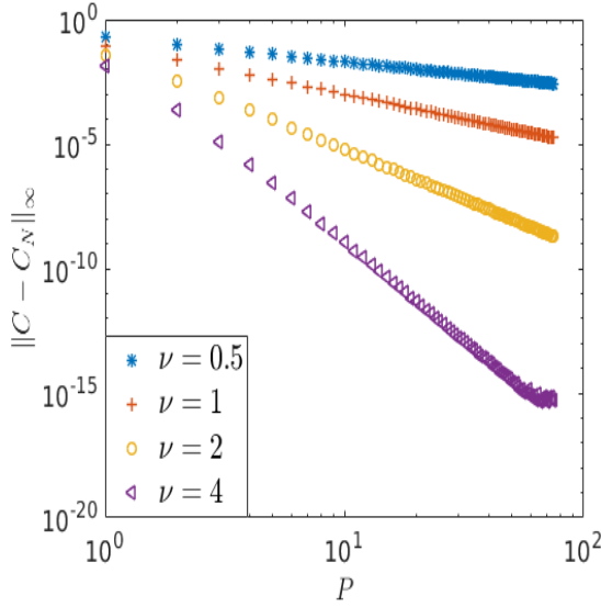
Figure 5: \|C - C_N\|_\infty with respect to P .
