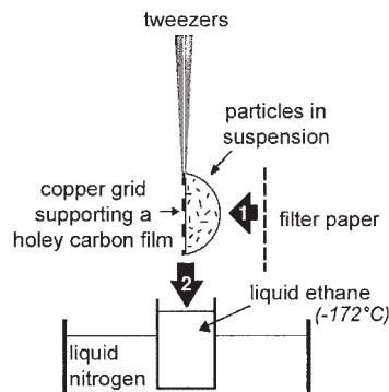
Figure 1 Principle of the fast-freezing protocol to prepare thin vitrified specimens for cryo-TEM.
