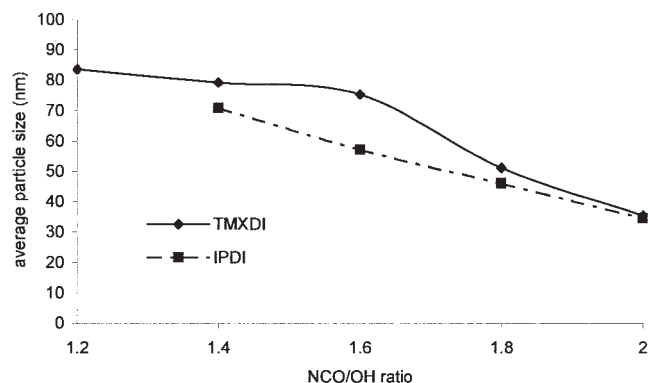
Figure 13 Effect of [NCO]/[OH] ratio on the average particle size of dispersions (see Table VIII).
