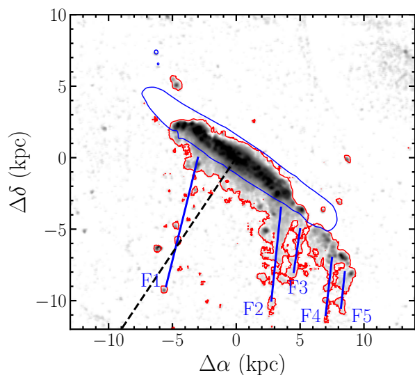
Fig. 4. CFHT/VESTIGE H\alpha image of NGC4330 shown in Figure 3. The blue contour is drawn from the r -band image at the 23^{\text{rd}} mag/arcsec 2 and identifies the region of the galaxy disc. In the text we refer to the H\alpha flux inside this region as the disc flux, and we refer to the H\alpha flux outside this region as the stripped flux in the tail. The black dashed line marks the separation between the upturn region (E of the centre) and the HI tail region (W of the centre). Five filaments of stripped gas are highlighted with blue segments and labelled F1 to F5 from east to west.
