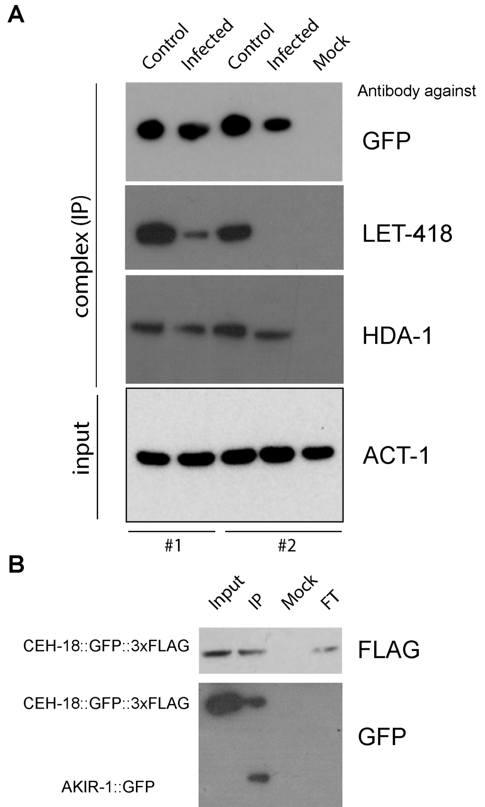
Fig 6. Validation of AKIR-1 interactors by Western blotting. A. Complexes immunopurified using an anti-GFP antibody from control or infected worms with a single copy AKIR-1::GFP insertion ( wt; ftSi12[pNP157(akir-1p)::AKIR-
