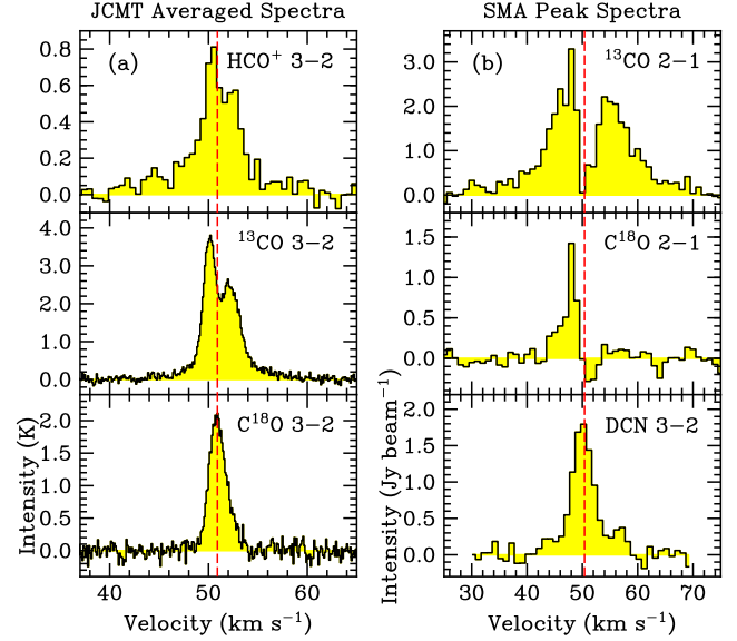
Figure 11. (a) JCMT \text{HCO}^+ (3 – 2), ^{13}\text{CO} (3 – 2), and \text{C}^{18}\text{O} (3 – 2) spectra averaged over clump C1. (b) SMA ^{13}\text{CO} (2 – 1), and \text{C}^{18}\text{O} (2 – 1) and DCN (3 – 2) spectra at the peak of SMA1.
