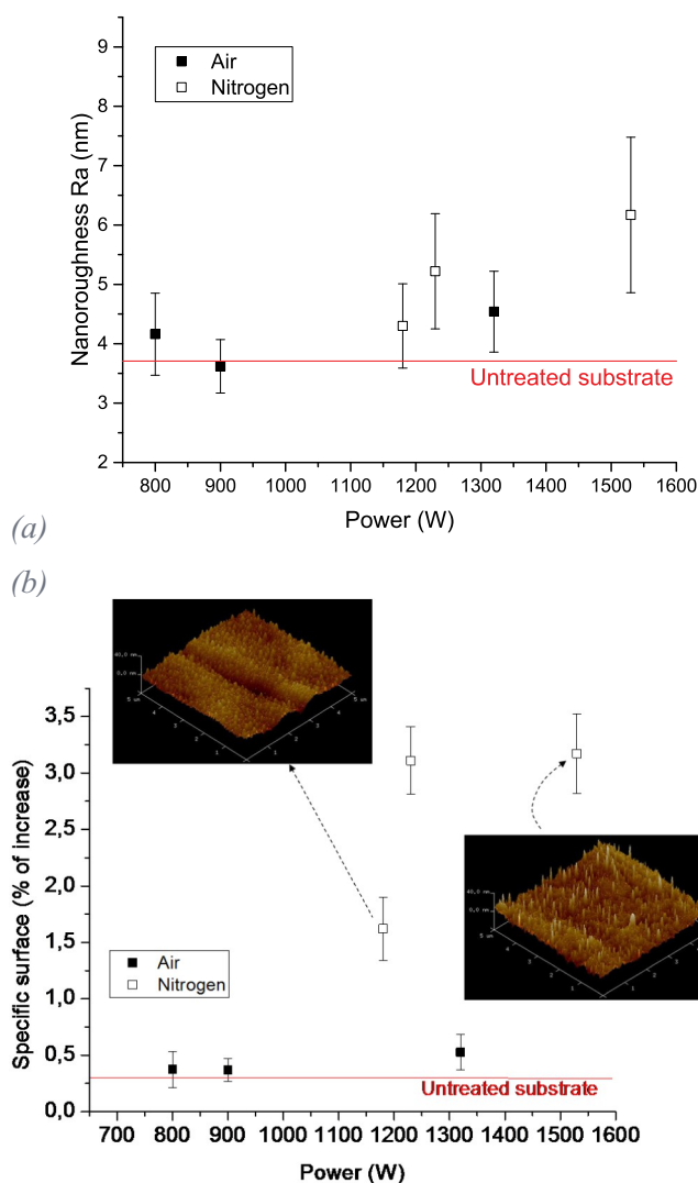
Fig. 9. (a) Nanoroughness and (b) specific surface evolution data obtained by AFM in Peak Force mode, relative to gas and plasma power. Values before plasma activation are represented by the continuous line.
