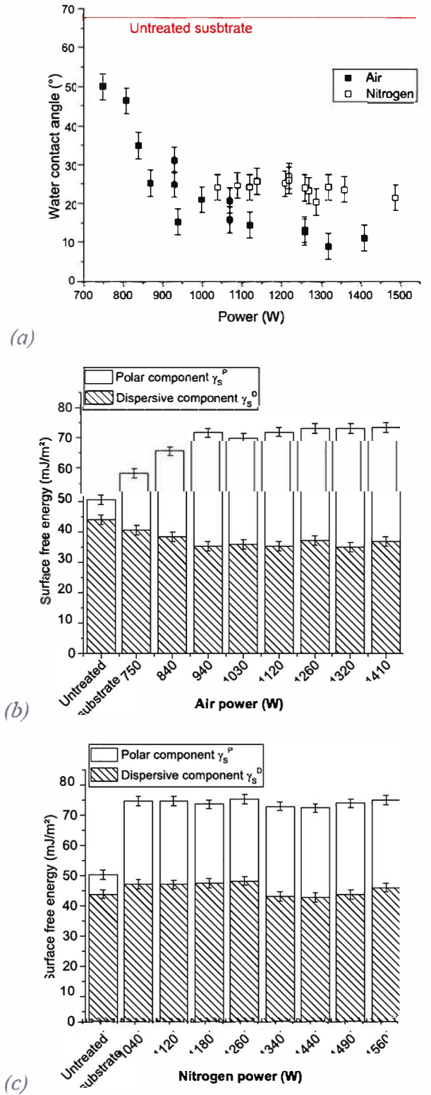
Fig. 6. (a) Water contact angles and surface free energies after (b) air or (c) nitrogen treatment relative to the plasma power.
