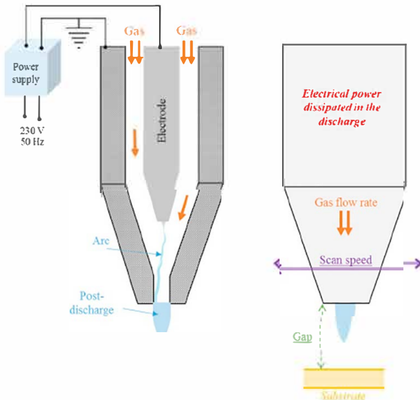
Fig. 1. Schematic representation of the experimental UL-SCAN device.
