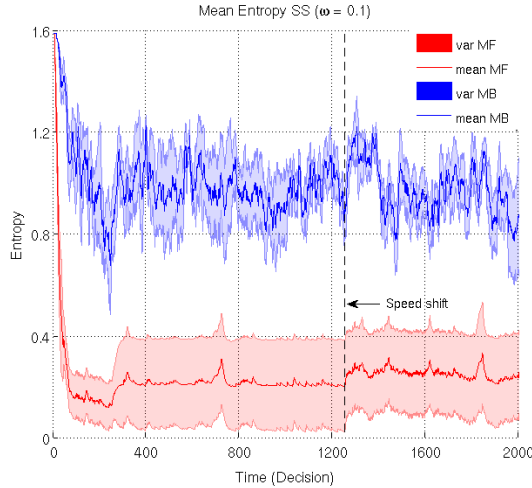
(a) Action distribution entropy.
