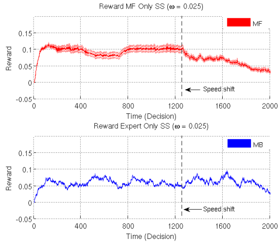
(b) Mean reward.
