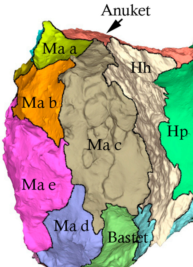
Fig. 21. The shape model showing the 5 sub-regions of Maat. Note the different surface appearances.
