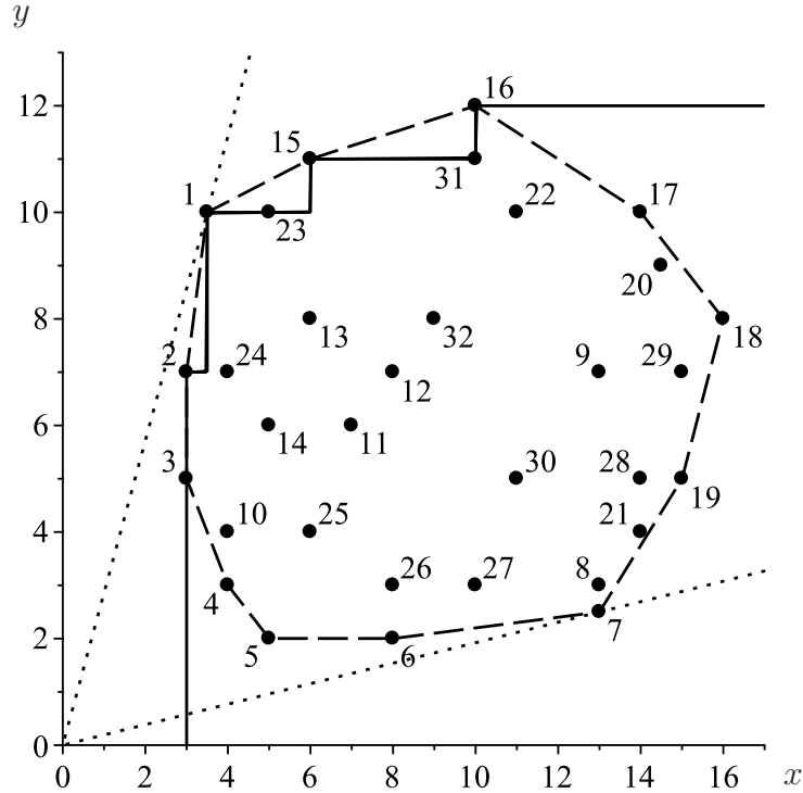
Figure 1: Different Hull operators Applied to the Same Set
