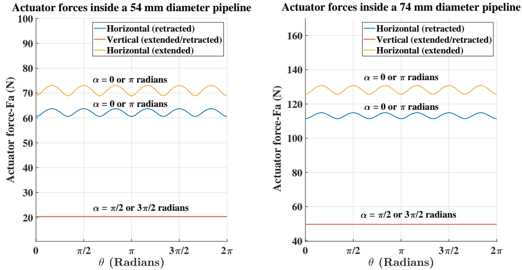
Figure 8. Front/Rear module actuator forces F_a inside 54 mm (left) and 74 mm (right) diameter pipelines for horizontal ( \alpha = 0 or \pi radians) and vertical ( \alpha = \pi/2 or 3\pi/2 radians) orientations.
