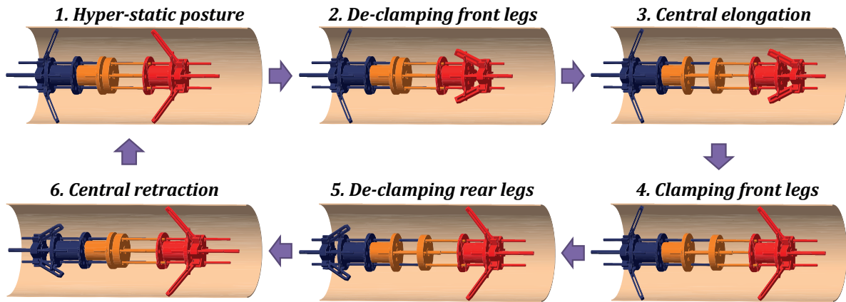
Figure 2. Demonstration of the six locomotion steps to attain caterpillar motion by the robot [20].
