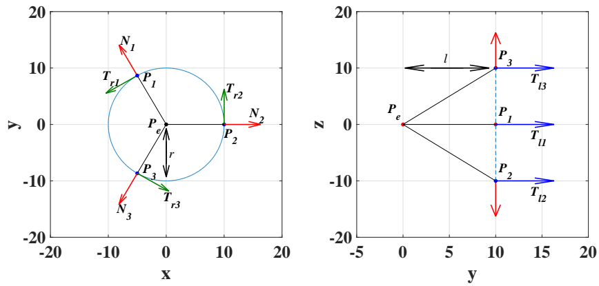
Figure 5. Schema of the contact forces during clamping as seen in x - y (left) and y - z (right) planes.
