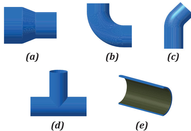
Figure 6. Possible profiles encountered by an inspection robot inside an industrial pipeline: (a) varying diameter; (b) curvature; (c) inclination; (d) branching; and (e) uneven surface walls [21].
