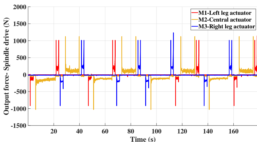
Figure 12. Experimental output forces in the spindle drive for vertical orientation ( \alpha= \pi/2 or 3\pi/2 radians) of pipeline.
