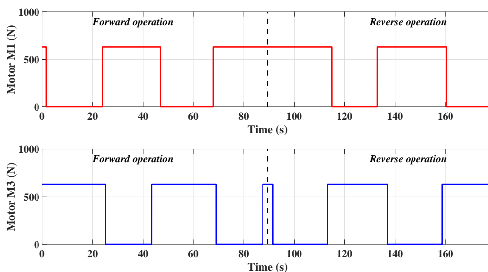
Figure 13. Clamping forces ( F_p ) between legs of robot and PVC test pipe from experiments.
