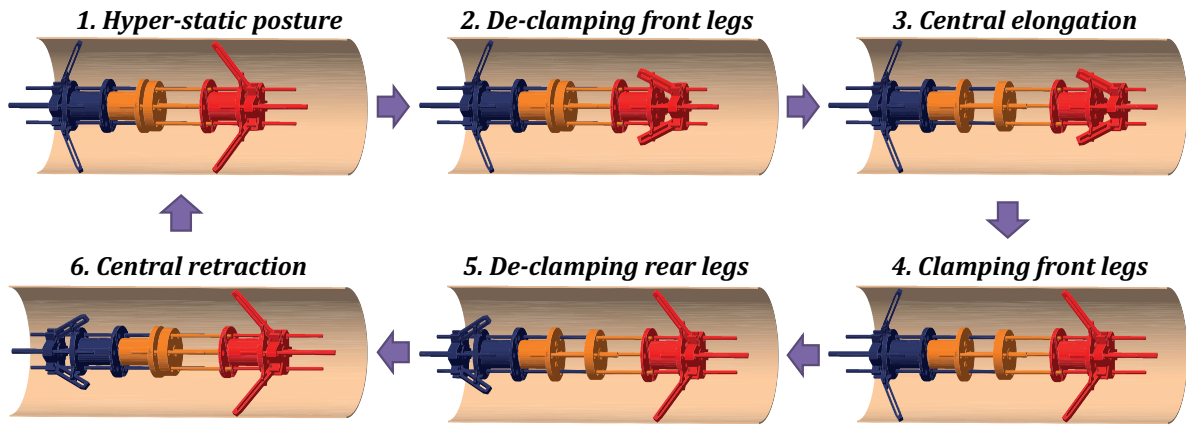
Figure 2. Demonstration of the six locomotion steps to attain caterpillar motion by the robot [20].
