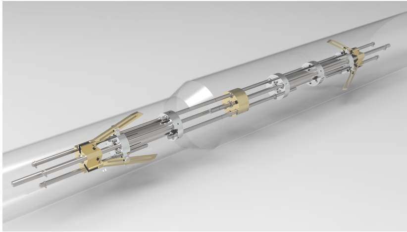
Figure 7. Digital model of the robot in CATIA software [17].
