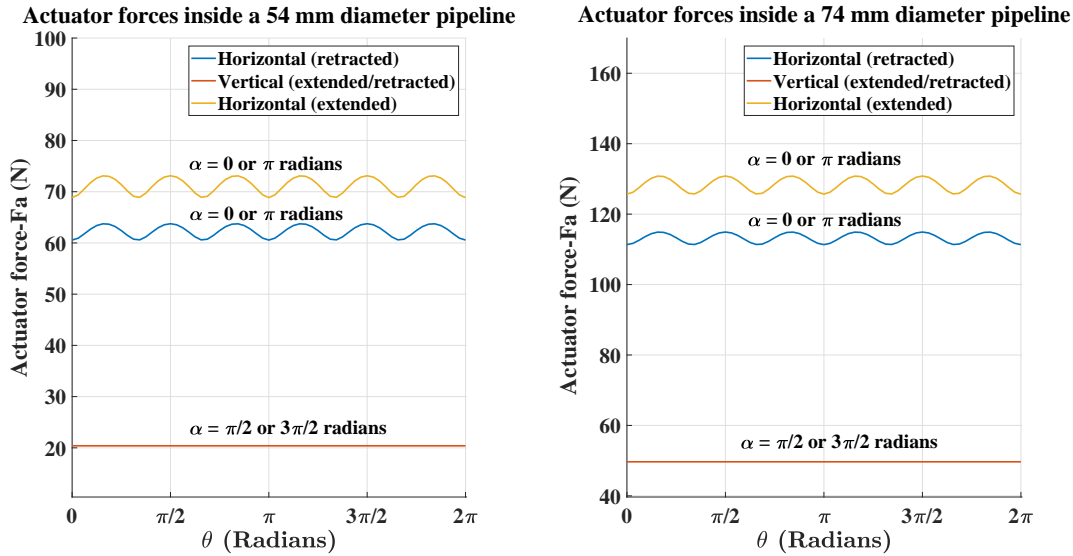
Figure 8. Front/Rear module actuator forces F_a inside 54 mm (left) and 74 mm(right) diameter pipelines for horizontal ( \alpha = 0 or \pi radians) and vertical ( \alpha = \pi/2 or 3\pi/2 radians) orientations.
