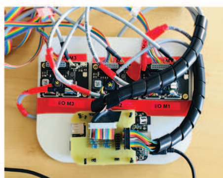
(C) ESCON controllers and BeagleBone black
