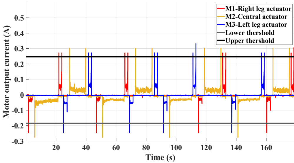
Figure 10. Output current of EC-motors from experiments.
