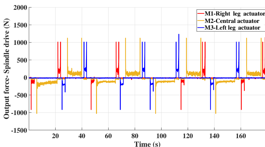
Figure 11. Experimental output forces in the spindle drive for horizontal orientation ( \alpha=0 or \pi radians) of pipeline [27].
