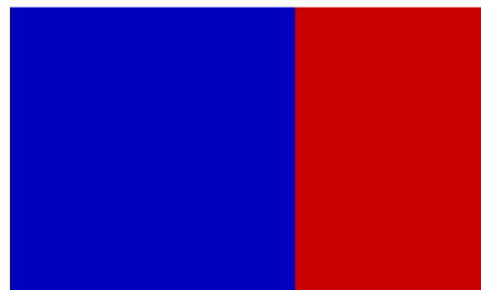
Concentration of MinA at t = 40\text{ s}
