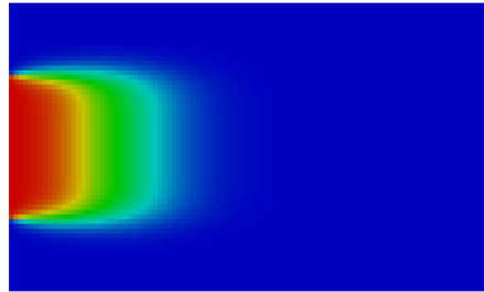
Concentration of \text{CO}_2 at t = 40\text{ s}
