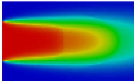
Concentration of CO_2 at t = 200 s
