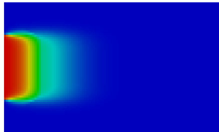
Concentration of H^+ at t = 40\text{ s}
