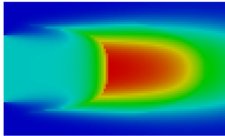
Concentration of HCO_3 at t = 200 s
