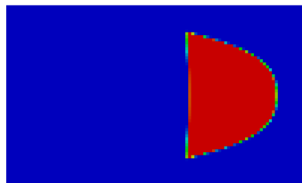
Concentration of MinB at t = 200 s
