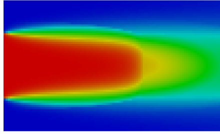
Concentration of H^+ at t = 360 s
