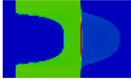
Concentration of Calcite at t = 200 s
