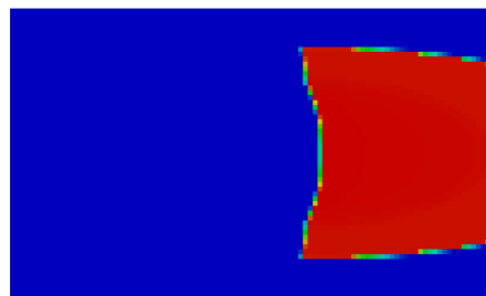
Concentration of MinB at t = 360 s
