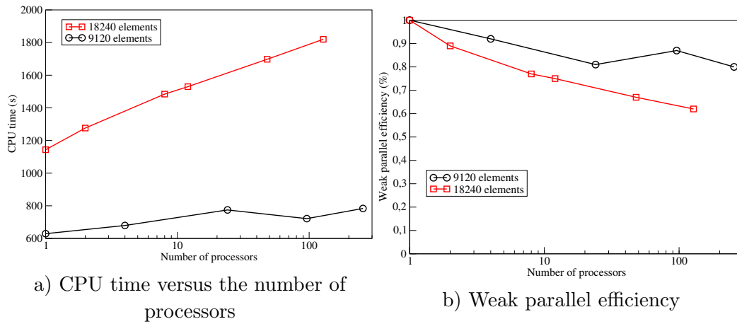
Figure 18: CPU time and weak parallel efficiency as a function of the number of processors.
