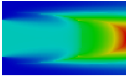
Concentration of HCO_3 at t = 360 s
