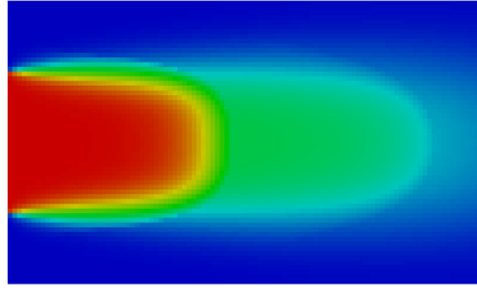
Concentration of H^+ at t = 200 s
