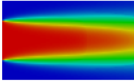
Concentration of CO_2 at t = 360 s
