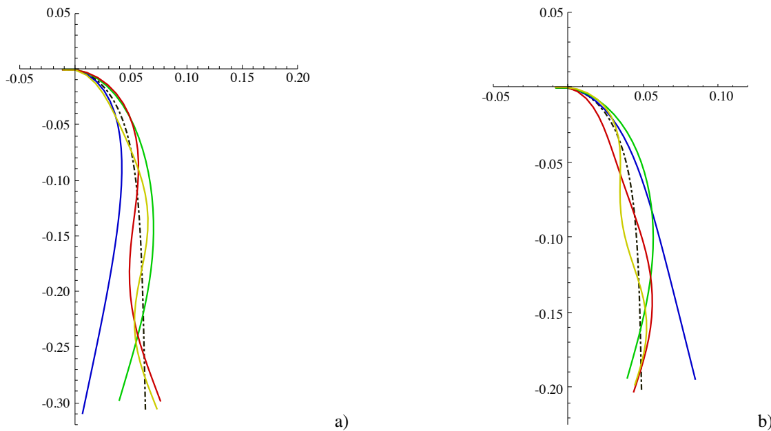
Fig. 7 First four natural modes (solid lines) around the global equilibrium shape (dot-dashed line). Paper beam a ; PET beam with a mass on the tip b . Legend: blue line corresponds to the first mode; green line to the second mode; red line to the third mode; yellow line to the fourth mode.
