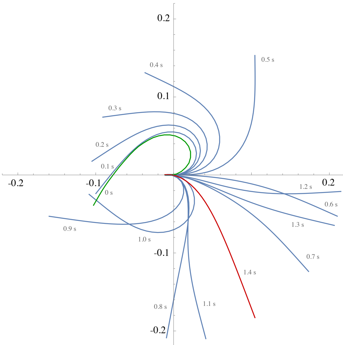
Fig. 14 Stroboscopic motion of the PET beam without mass on the tip. The initial shape is highlighted in green and the final one in red. The label near each configuration represents the attained time for the shown configuration.
