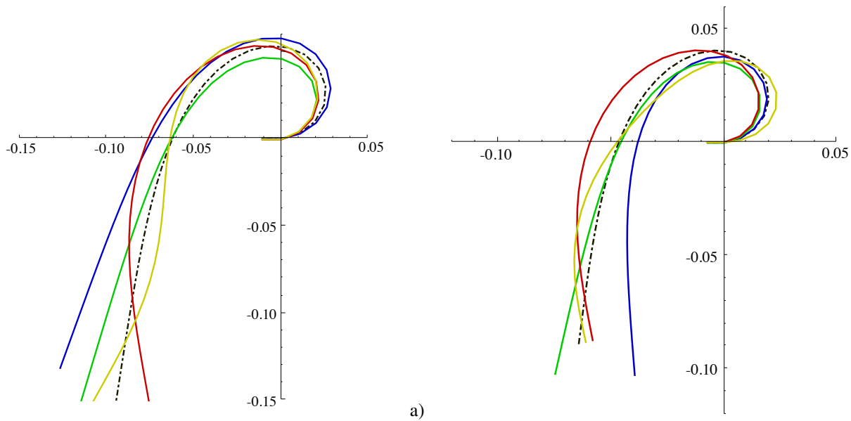
Fig. 8 First four natural modes (solid lines) around the local 'curled' equilibrium shape (dot-dashed line). Paper beam a ; PET beam with a mass on the tip b . Legend: blue line corresponds to the first mode; green line to the second mode; red line to the third mode; yellow line to the fourth mode.
