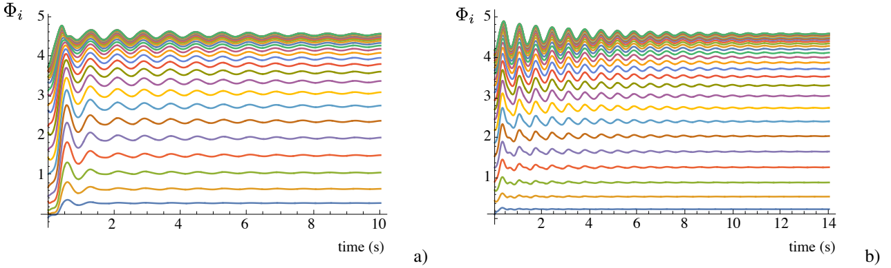
Fig. 10 Time history of the Lagrangian coordinates, \Phi_i(t) , around the curled equilibrium configurations for the paper case a , and for the PET case b . Their plots result in an increasing order from the \Phi_1(t) to \Phi_{Ne}(t) .
