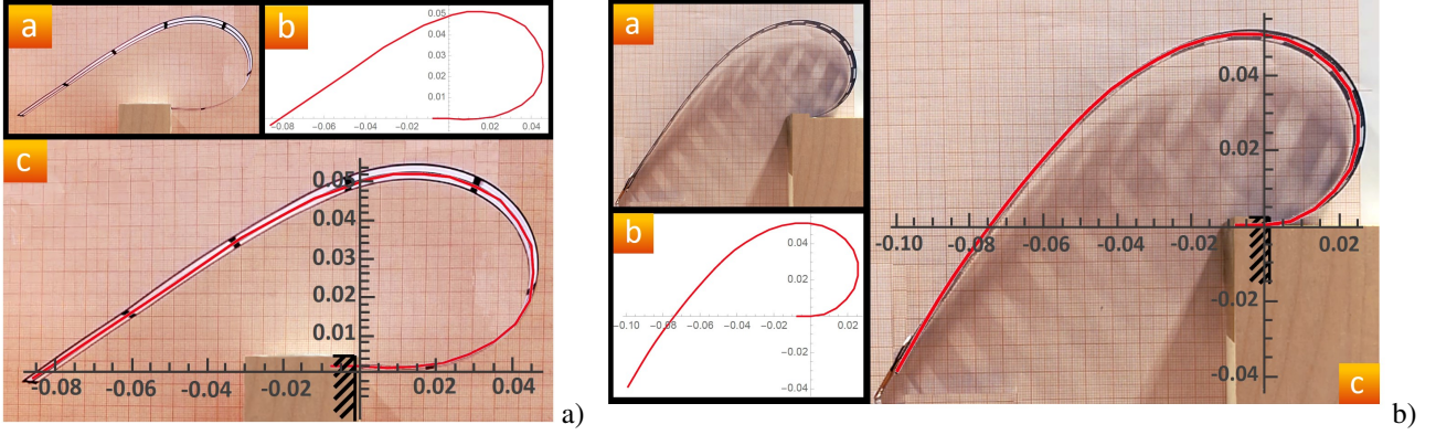
Fig. 9 Experimentally imposed and numerically evaluated initial configurations: paper beam a ; PET beam with a mass on the tip b .
