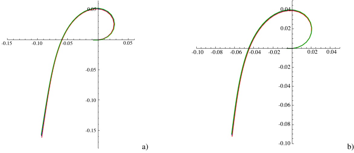
Fig. 6 Curled stable equilibrium configurations with different constitutive laws: quadratic elastic potential (blue solid line); cosine elastic potential (red solid line); hyperbolic cosine elastic potential (green solid line). Paper beam a ; PET beam with a tip mass b . The curled stable equilibrium configurations represented here are discretized in N_e = 40 elements.
