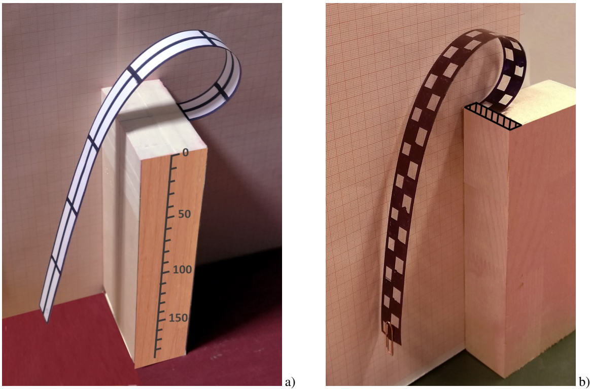
Fig. 3 Stable nonstandard 'curled' equilibrium shapes: paper beam a ; PET beam with a mass on the tip b .
