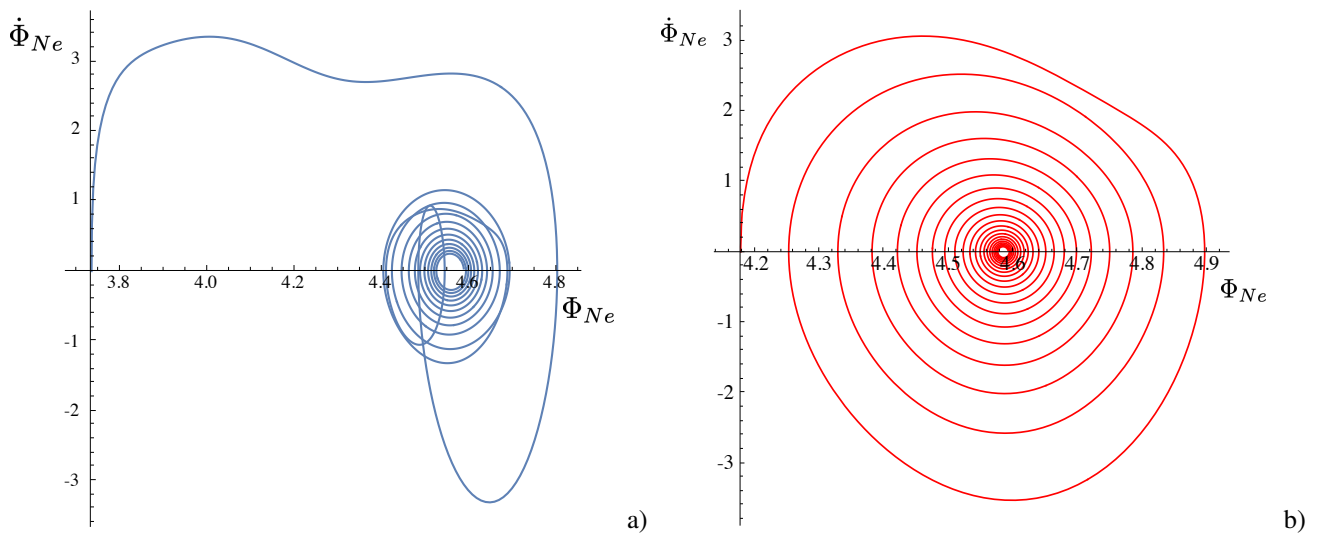
Fig. 13 \dot{\Phi}_{Ne} vs \Phi_{Ne} phase paths of the paper case a , and of the PET case b .
