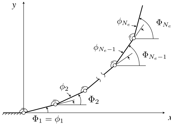
Fig. 2 Hencky-type lumped mass-spring model for a highly flexible beam.
