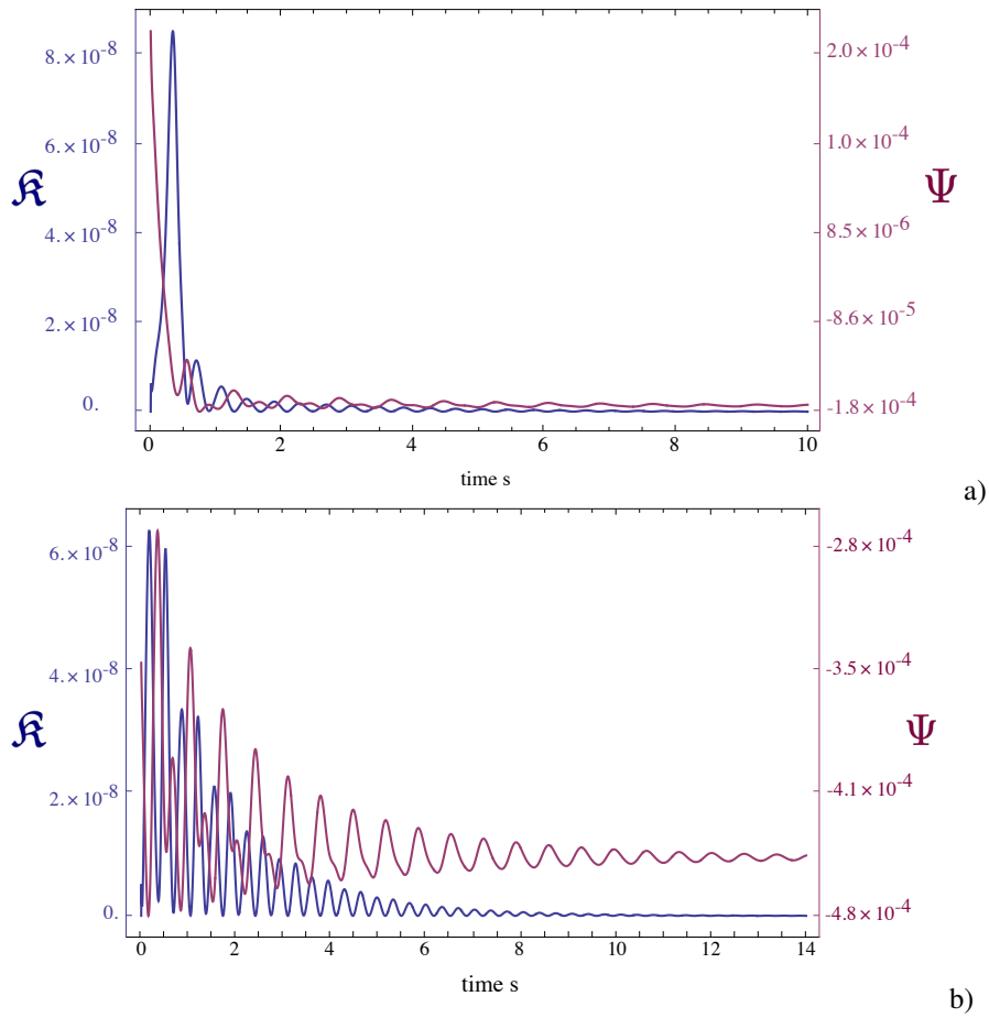
Fig. 12 Kinetic \mathcal{R} (blue solid line) and potential energy \Psi (purple solid line) vs time graphs for the paper case a , and for the PET case b .
