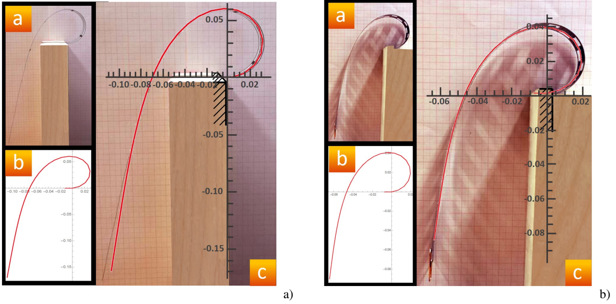
Fig. 5 Experimentally observed and numerically evaluated equilibrium configurations: paper beam a ; PET strip with a tip mass b .
