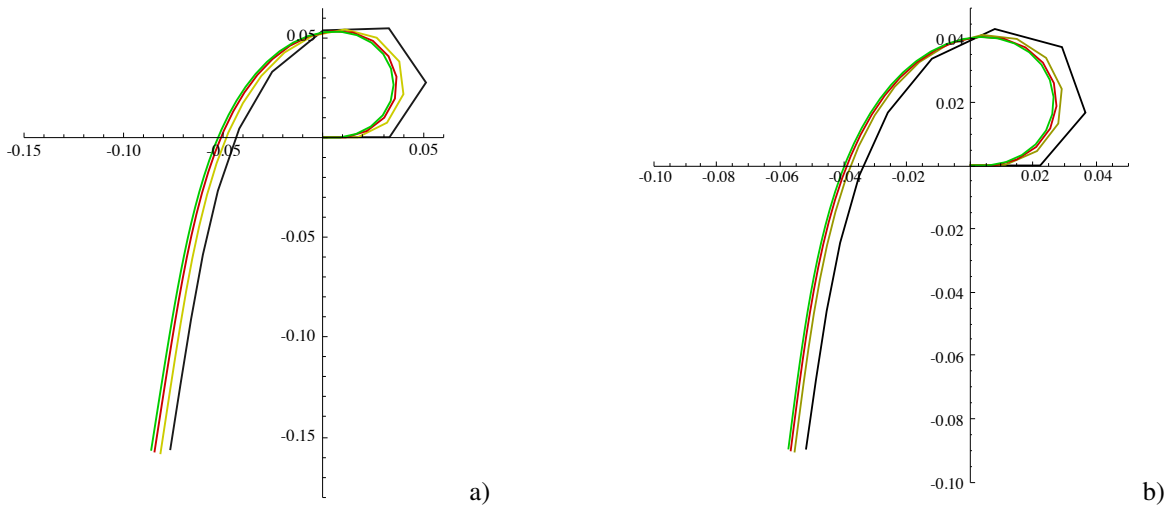
Fig. 4 Convergence analysis of curled stable equilibrium configurations obtained by numerical simulations: paper beam a ; PET beam with a mass on the tip b . The curled stable equilibrium configurations represented here are discretized in N_e = \{10, 20, 30, 40\} elements.
