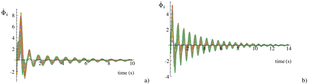
Fig. 11 Time history of the angular velocities, \dot{\Phi}_i(t) for the paper case a , and for the PET case b .
