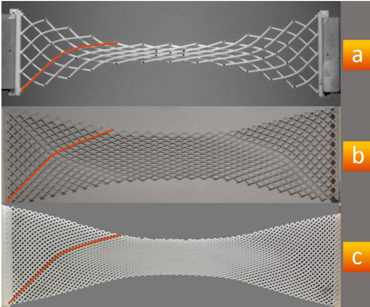
Fig. 1 Some illustrative examples of pantographic structures under a bias test varying the density of the fibers.
