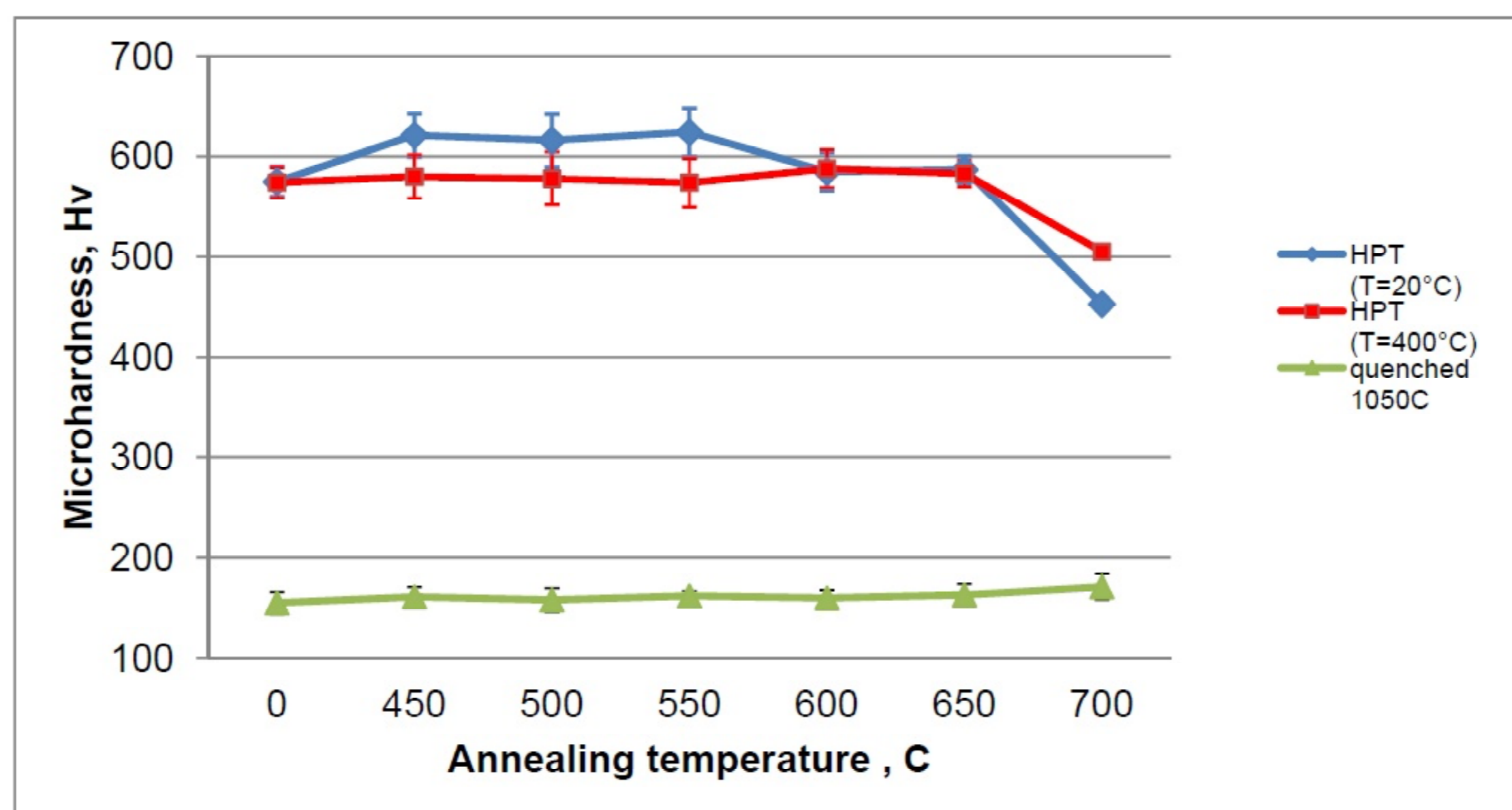
Fig. 6. Microhardness after 1 hour annealing at different temperatures.
