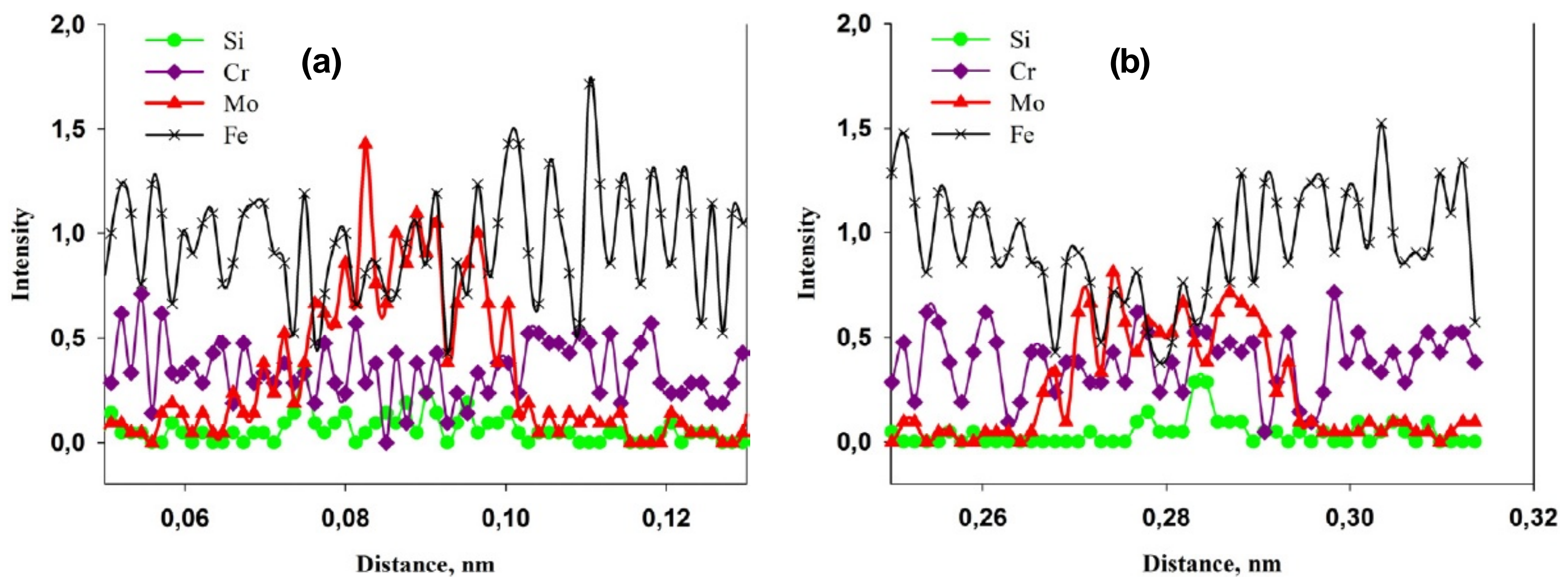
Fig. 5. STEM-EDS intensity profiles across precipitates from Fig. 4b #1(a) and #2 (b) in the austenitic stainless steel after HPT at 400 °C and annealing at 700 °C for 10 min revealing their Mo-Cr-Si composition.
