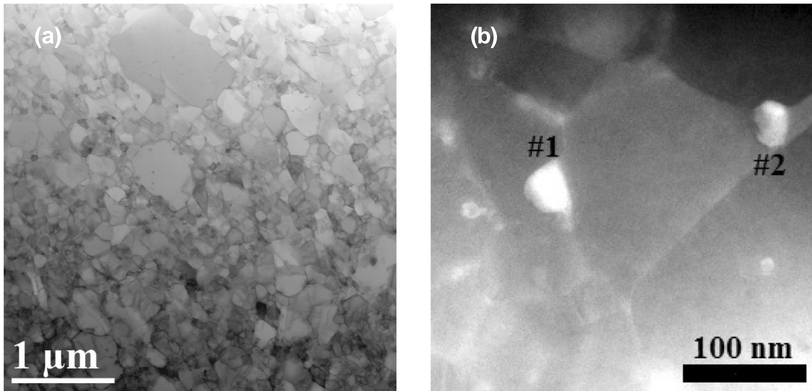
Fig. 4. STEM microstructure of the UFG steel produced by HPT at 400 °C after annealing at 700 °C for 10 min showing grain growth and formation of precipitates inside grains (a) and at grain boundaries (b).
