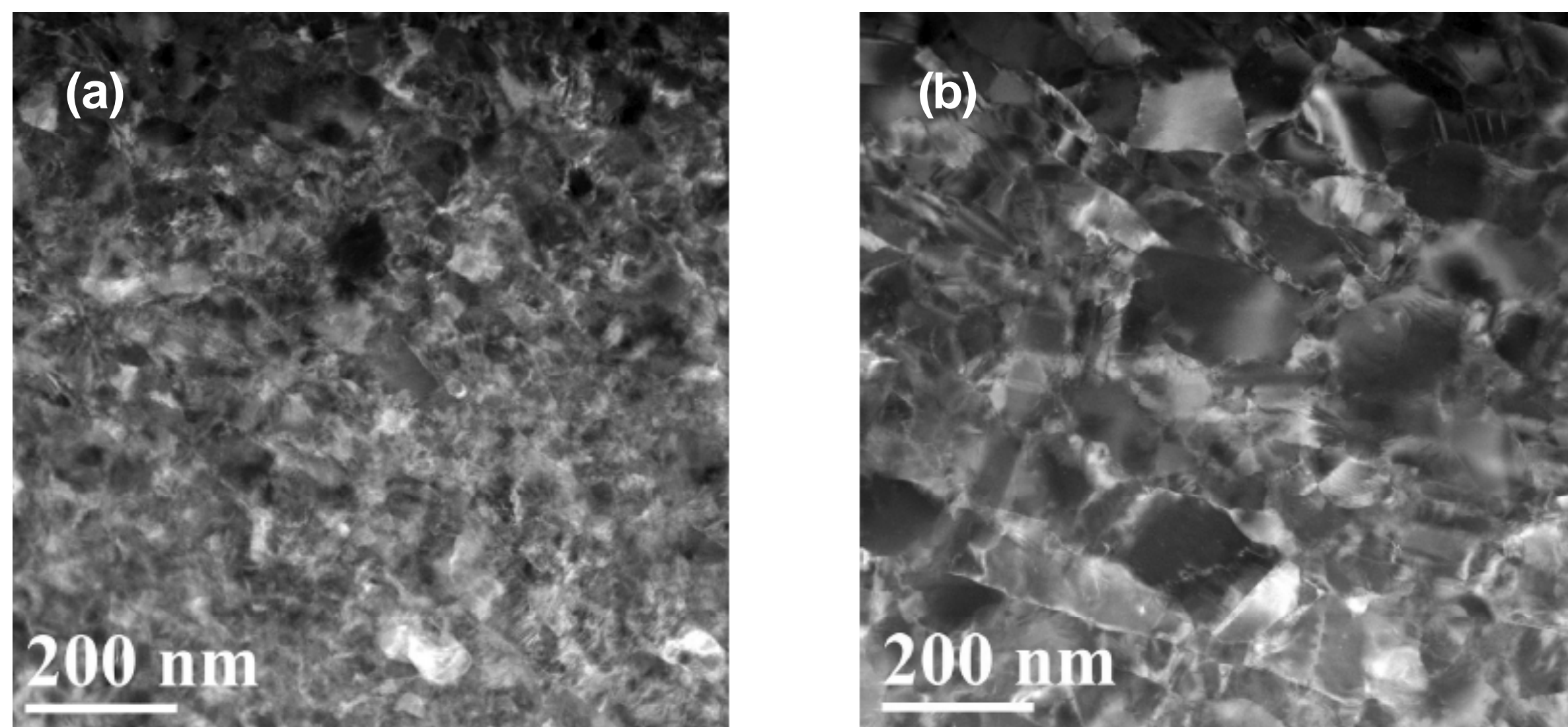
Fig. 1. STEM dark field images of the microstructure of the UFG steel produced by HPT at (a) – room temperature, (b) – T = 400\text{ }^{\circ}\text{C} .
