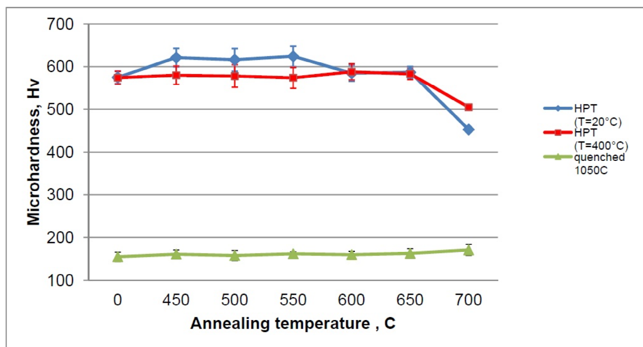
Fig. 6. Microhardness after 1 hour annealing at different temperatures.
