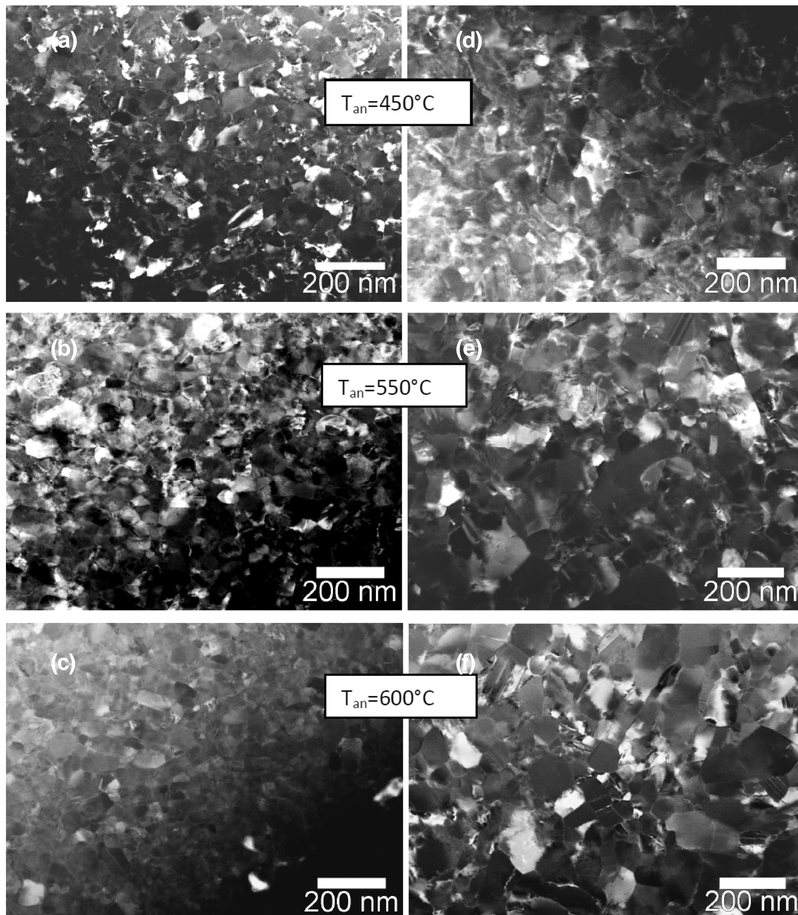
Fig. 3. STEM images of microstructure of an UFG austenitic stainless steel produced by HPT at room temperature (a-c) and at 400 °C (d-f) after 1 hour annealing at 450 °C (a,d), 550 °C (b,e), 600 °C (c,f).
