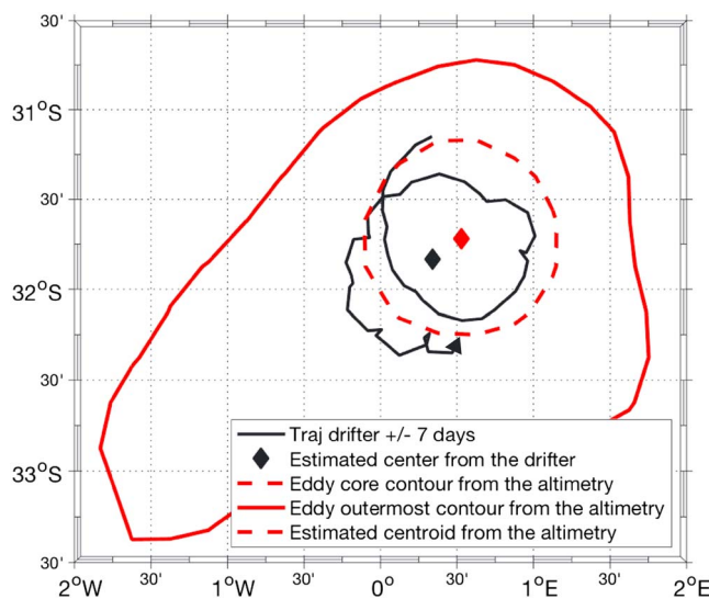
Figure 6. Example of cross detection of eddies for 12 December 2012 where an eddy identified from a surface drifter trajectory by LU16 (in black with a diamond symbol locating its center) and an anticyclone detected in the TOEddies Atlas (red contours for its outer limit and its maximum speed core with a red diamond symbol locating its center) overlap.
