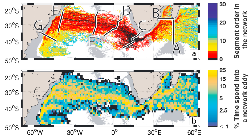
Figure 10. (a) Whole set of Agulhas Ring Eddy Network trajectories (from order 0 to maximum order 29). The color of the trajectories is related to their order. The black color is for order 0, which we defined as the main trajectories for the Agulhas Rings. Seven sections (A–G) were used to derive the Agulhas Rings properties across the basins. (b) Percentage of time each 1^\circ \times 1^\circ grid cell is within an Agulhas Ring Eddy Network trajectory. The gray shading in each figure represents water depths less than 3,500 m in the ETOPO2 data set (Smith & Sandwell, 1997).
