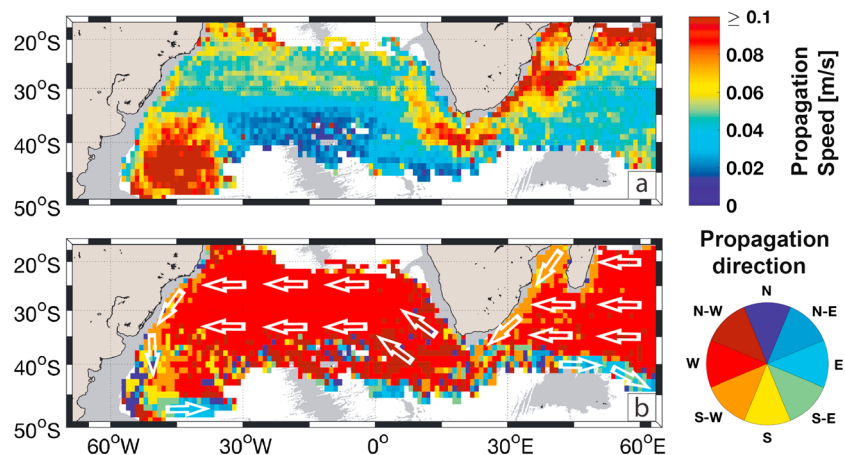
Figure 12. (a) Median of the propagation velocity of the Agulhas Ring Eddy Network (m/s) and (b) associated main propagation direction. These properties are calculated on a 1^\circ \times 1^\circ grid, and the propagation direction is computed from the eddy positions 1 week apart. Schematic white arrows have been added in the bottom panel to highlight the main propagation direction. The gray shading in each figure represents water depth shallower than 3,500 m in the ETOPO2 data set (Smith & Sandwell, 1997).
