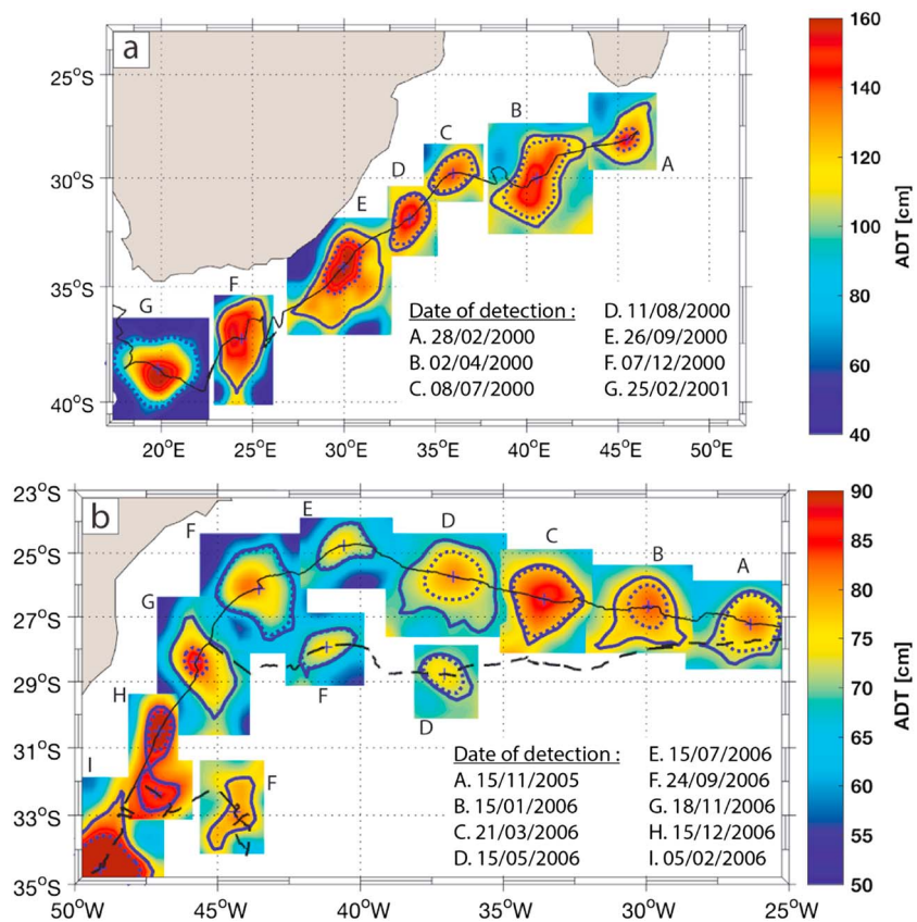
Figure 16. Composite figure of the order 0 Agulhas Ring Eddy Network starting the most to the east (a) and ending the most to the west (b). Snapshots on selected dates are given, in blue the eddy centroid (cross symbol), the absolute dynamic topography (ADT) contour associated with the maximum speed (dotted), and the outermost ADT (solid line) contours. The trajectory of panel (b) interacts with two order 1 trajectories whose paths are drawn in dashed lines.
