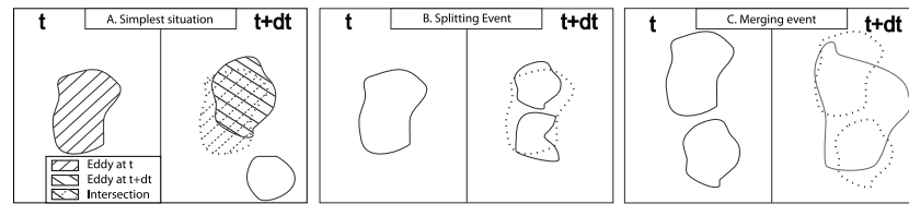
Figure 3. Schematic diagram of the eddy tracking step of the algorithm. (a) Simplest situation where a single eddy is identified at the two different time intervals, t and t + dt . The area of the two eddy occurrences and their overlapping surface are shown, the latter in the form of a hatched surface. (b) Splitting event. (c) Merging event. Although the overlap threshold is applied in (b) and (c), these areas have not been represented to ensure readability of the figures.
