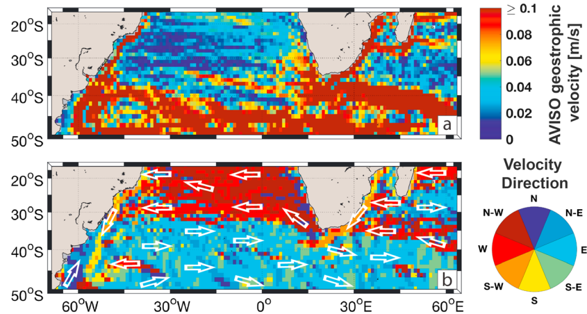
Figure 13. (a) Mean surface geostrophic velocity estimated from AVISO satellite altimetry (m/s) and (b) associated main direction. These properties are computed on a 1^\circ \times 1^\circ grid. Schematic white arrows have been added in the bottom panel to highlight the main velocity direction. The gray shading in each figure represents water depth less than 3,500 m in the ETOPO2 data set (Smith & Sandwell, 1997).
