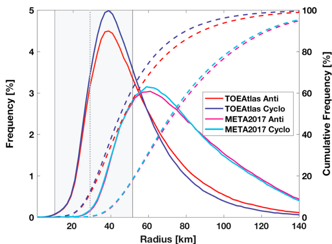
Figure 7. Histograms (solid lines) and cumulative frequency (dashed lines) of the eddy R_{max} for TOEddies (red and blue lines) and META2017 (pink and light blue lines) computed over 2-km intervals. The vertical dotted line is the mean first baroclinic Rossby radius ( L_R ) of deformation in the area and the gray dashed area limits the 10th and 90th percentiles. The baroclinic Rossby radius of deformation is computed by applying the Chelton et al. (1998) method on the World Ocean Database (Boyer et al., 2013) averaged over 7 years (i.e., 2005 to 2012).
