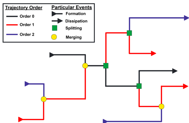
Figure 4. Schematic of a simple network of trajectories up to order 2. This network is characterized by four formations, four disappearances, and three merging and splitting events. With each merging and splitting, the cost function is applied to follow the main trajectory by associating a segment with a higher order.
