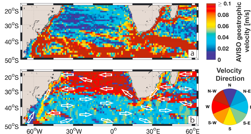
Figure 13. (a) Mean surface geostrophic velocity estimated from AVISO satellite altimetry (m/s) and (b) associated main direction. These properties are computed on a 1^\circ \times 1^\circ grid. Schematic white arrows have been added in the bottom panel to highlight the main velocity direction. The gray shading in each figure represents water depth less than 3,500 m in the ETOPO2 data set (Smith & Sandwell, 1997).
