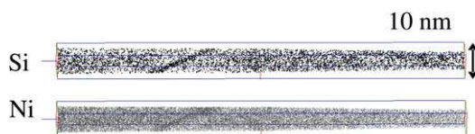
Fig. 7. 3D reconstruction of a volume of ion-irradiated nanostructured CW 316 SS analysed with LATAP. Si and Ni are represented. A grain boundary is clearly visible.
