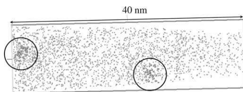
Fig. 4. 3D reconstruction of a volume of 316 SS ion irradiated to 5 dpa analysed. Only Si is represented. Thick atoms into black circles correspond to Si clusters (Si concentration >4 at.%).
