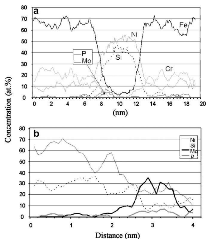
Fig. 2. (a) Concentration profile along a cluster. Fe, Ni, Cr, Si, Mo and P are represented. (b) Zoom of the P and Mo segregation (left part profile (a)).
