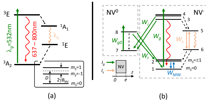
Fig. 1. Energy diagram of the NV center. (a) Level scheme of the \text{NV}^- center. As shown in the insert, the ground state ^3A_2 is split into m_S = 0 and m_S = \pm 1 sublevels due to spin-spin interaction and an external magnetic field applied to the NV center lifts the m_S = \pm 1 degeneracy. The \text{NV}^- center is spin polarized into m_S = 0 by optical pumping at \lambda_g = 532 \text{ nm} . The resonance zero-phonon wavelength of the singlet transition is \lambda_s = 1042 \text{ nm} . Typical lifetimes of the ^3E and ^1E levels are respectively 13 ns and 600 ns. (b) Description of the photodynamics between the spin sublevels of the \text{NV}^- and \text{NV}^0 ground and excited electronic states. W_g is the pumping rate associated to the \text{NV}^- and W_{g0} that of the \text{NV}^0 . W_s is the transition rate of the IR resonance. W_i and W_r are respectively the ionization and recombination rates of the \text{NV}^- \rightleftharpoons \text{NV}^0 transition. W_{\text{MW}} is the m_S = 0 \rightleftharpoons m_S = \pm 1 transition rate induced by the resonant microwave field. The insert shows the pump (green) and signal (IR) configuration, with propagation through the diamond plate of thickness e .
